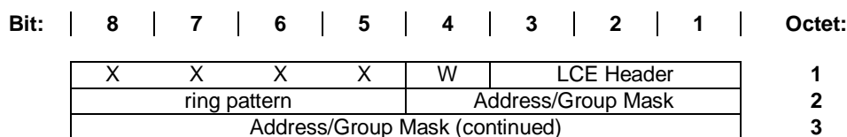
Figure 100: Short format message for collective or group ringing request
