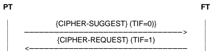
Figure H.6: PT initiated cipher switching, case 1
