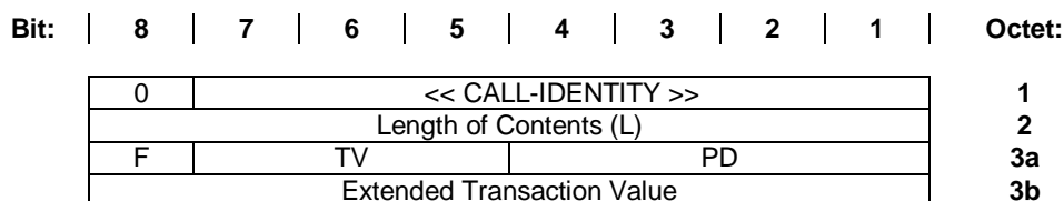
Figure 30: CALL-IDENTITY information element
