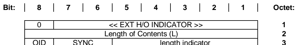
Figure 98: EXT H/O INDICATOR information element
