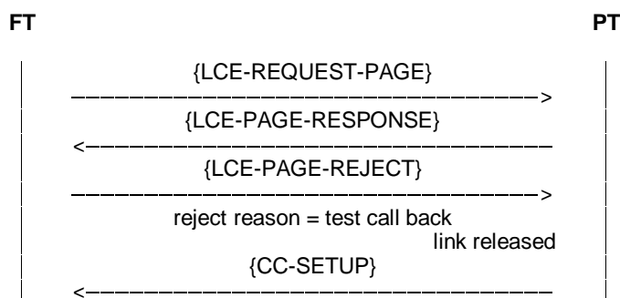
Figure 128: Test call back procedure
