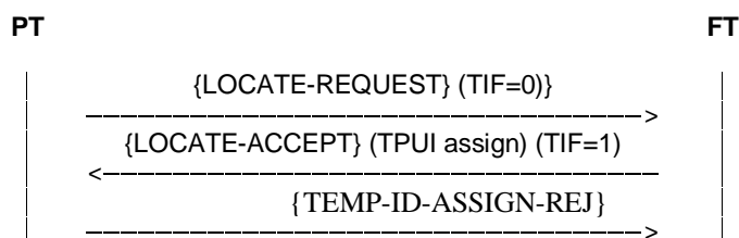
Figure H.5: TIF allocation, case 2
