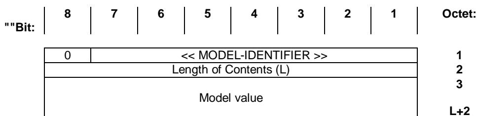
Figure 91: MODEL IDENTIFIER information element
