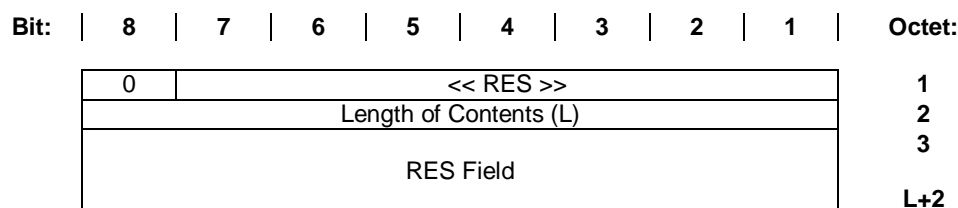
Figure 77: RES information element
