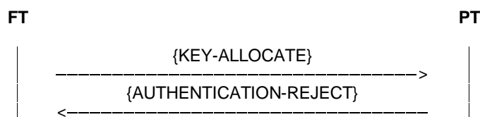
Figure 122: Unsuccessful key allocation procedure
