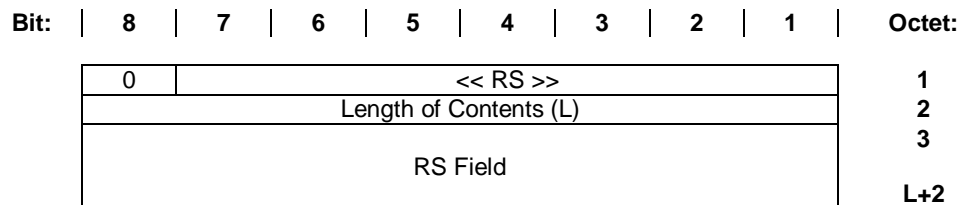
Figure 78: RS information element
