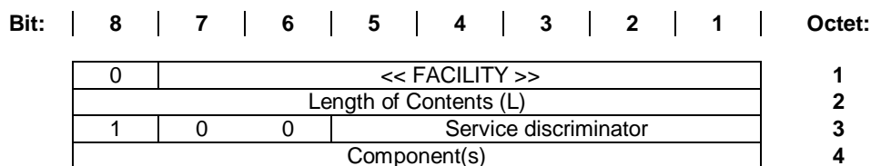
Figure 39: FACILITY information element
