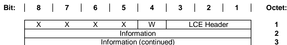
Figure 99: Short format message structure
