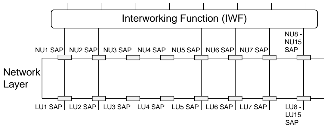
Figure 1b: C-plane model
