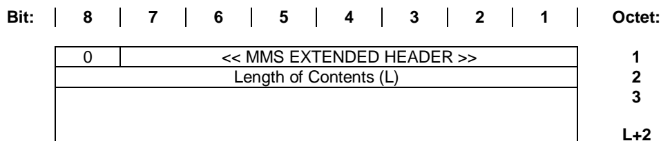
Figure 96: MMS EXTENDED HEADER information element
