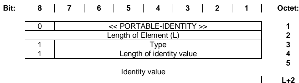
Figure 62: PORTABLE-IDENTITY information element
