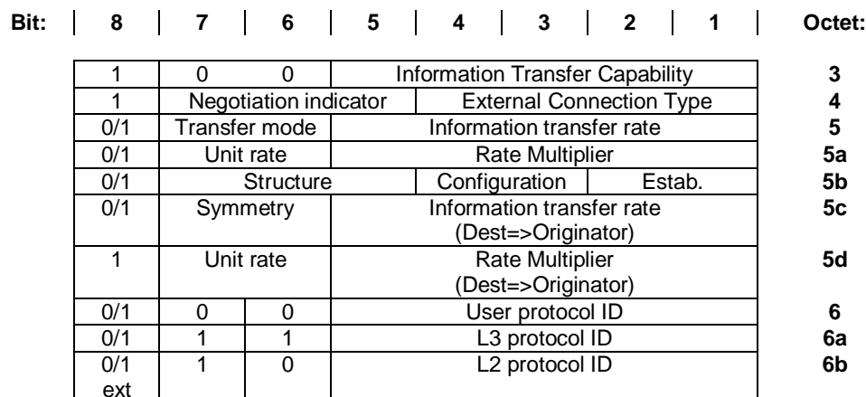
Figure 48: IWU-ATTRIBUTES information element for DECT standard coding
