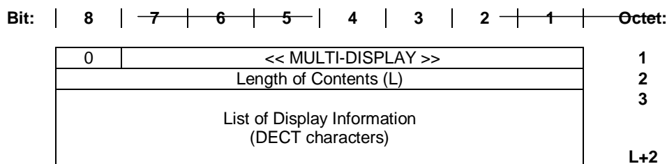
Figure 57: MULTI-DISPLAY information element
