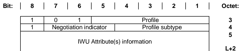
Figure 49: IWU-ATTRIBUTES information element for Profile defined coding standard
