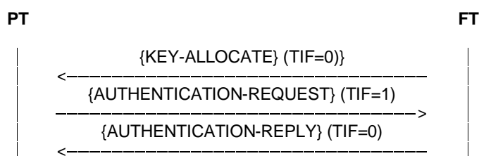
Figure H.9: Key allocation
