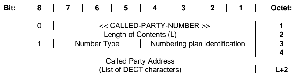
Figure 31: CALLED-PARTY-NUMBER information element
