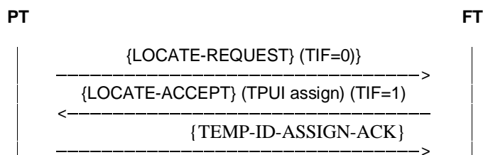
Figure H.4: TIF allocation, case 1
