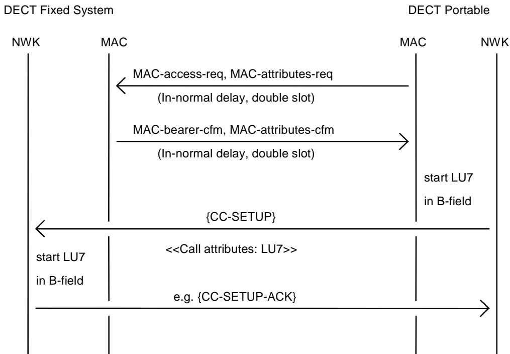
Figure 11.9.4.3.1.2: PT initiated call establishment with LU7
