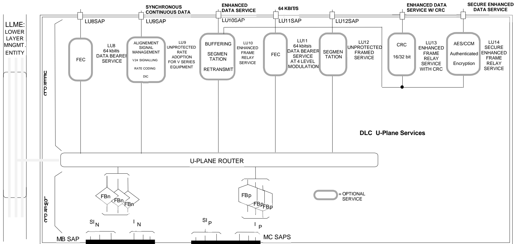
Figure 4.3.1: U-plane model
