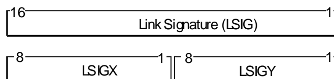
Figure 7.10.1: Link signature
