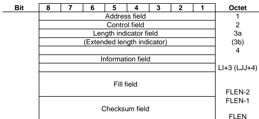
Figure 6.1.0.1: Frame format type FA
