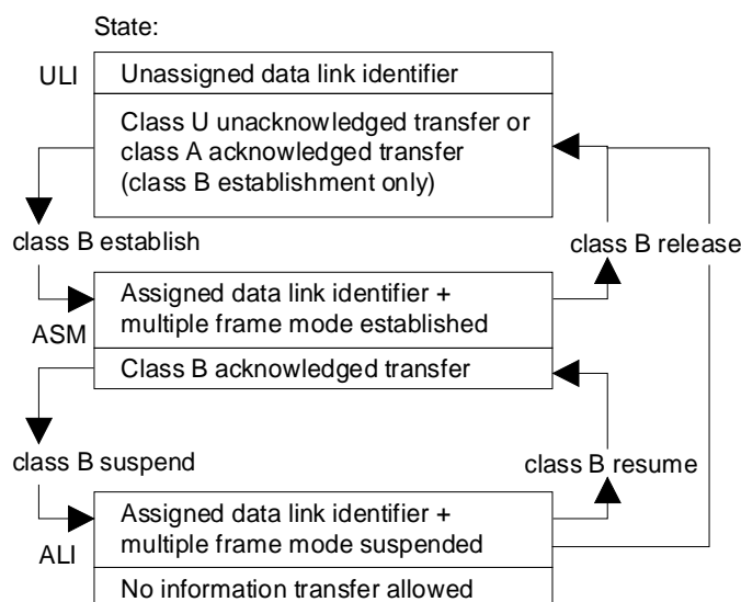
Figure 5.1.3.2.1: LAPC states
