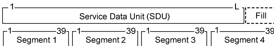
Figure 11.14.2.1.1: Example of segmentation in four full slot segments
