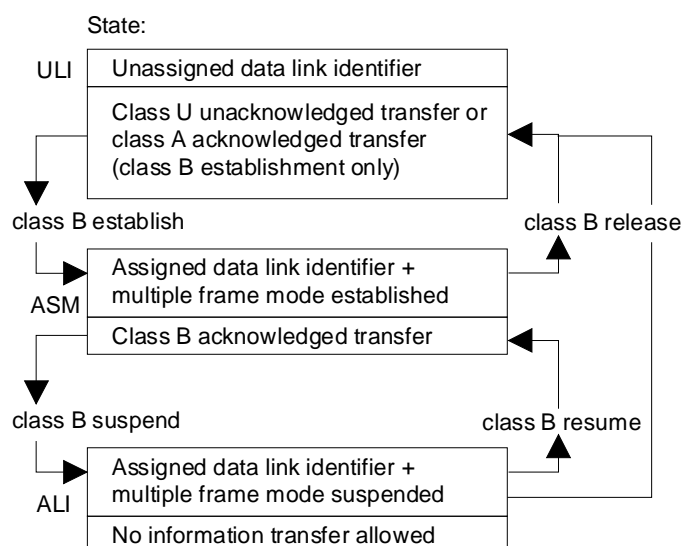
Figure 5.1.3.2.1: LAPC states
