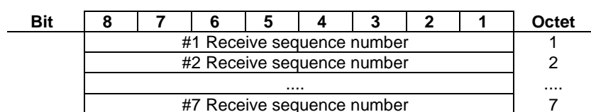
Figure 12.5.1.2: Frame format type FU4b
