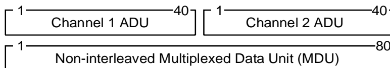
Figure 11.6.3.3.1: Example of non-interleaved packing (MCS Ref: N2/32)
