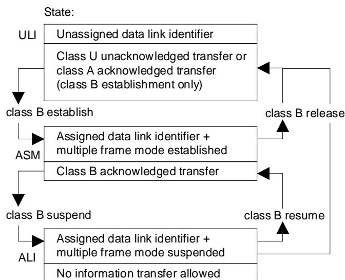
Figure 5.1.3.2.1: LAPC states
