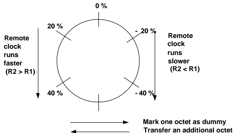
Figure 11.11.5.2.1: Phases diagram
