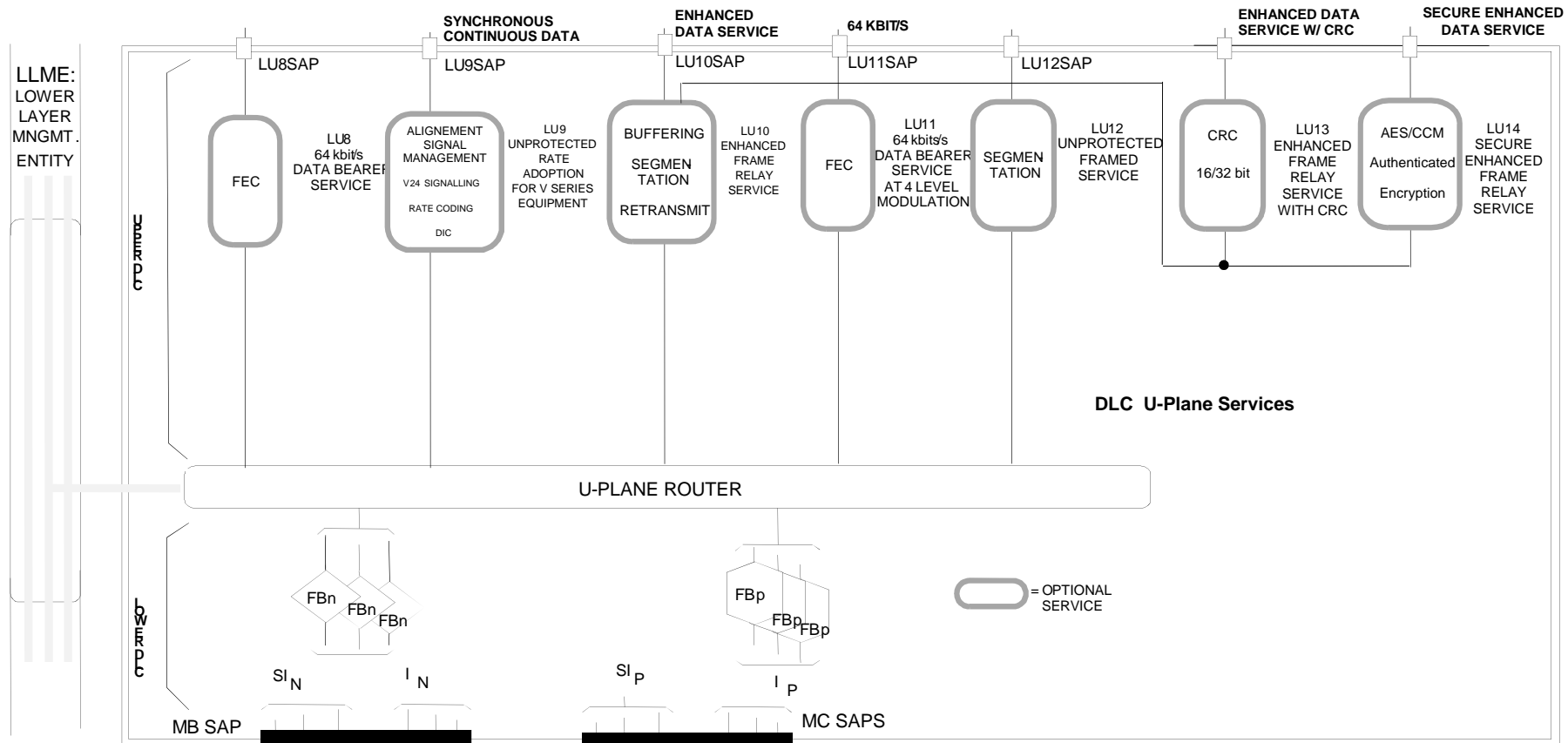
Figure 4.3.1: U-plane model
