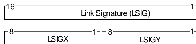
Figure 7.10.1: Link signature
