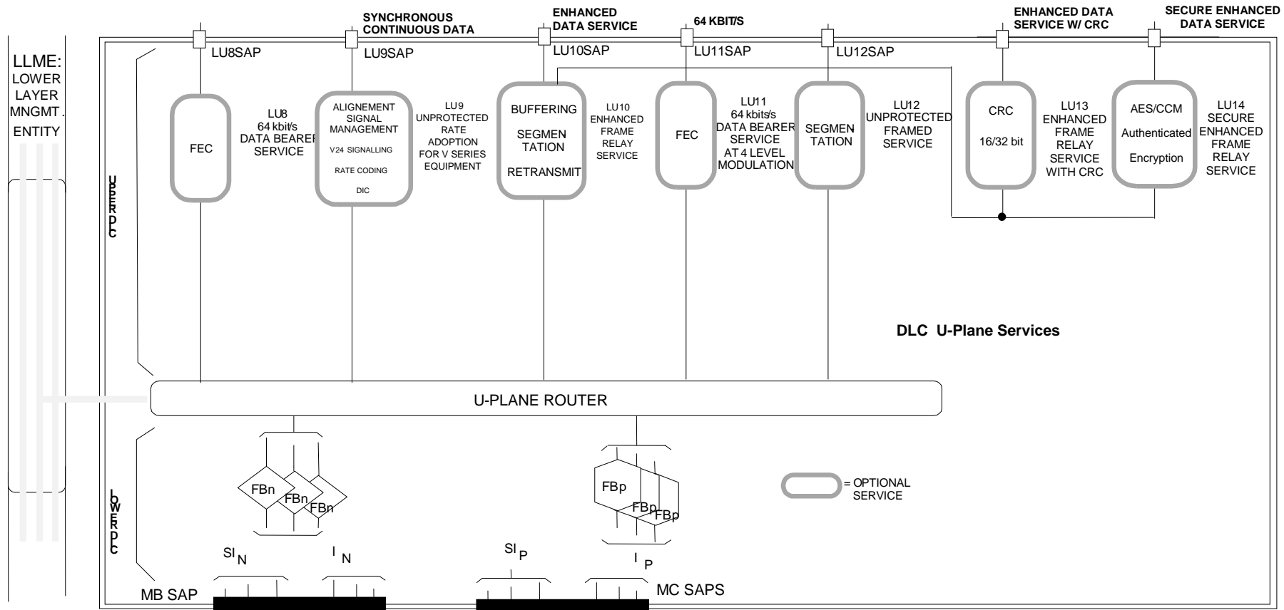
Figure 4.3.1: U-plane model
