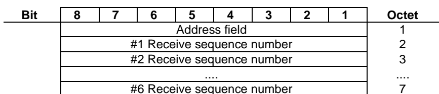
Figure 12.6.1.2: Frame format type FU5b
