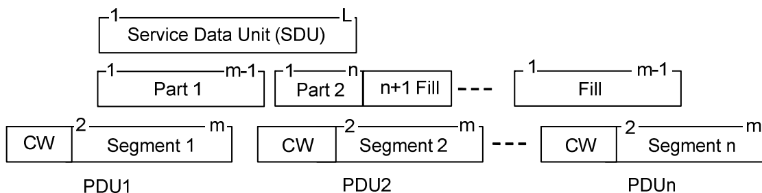
Figure 11.14.2.1: LU12 procedures
