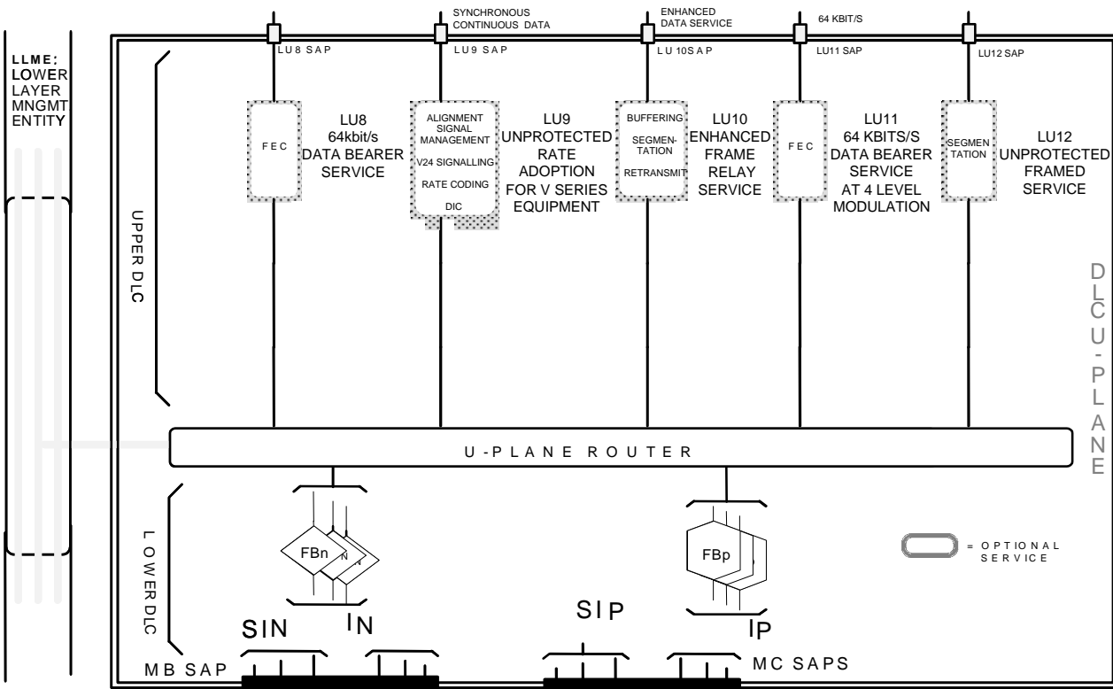
Figure 4.3.1: U-plane model
