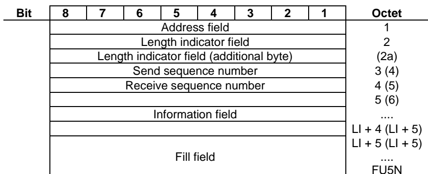
Figure 12.6.1.1: Frame format type FU5a
