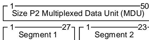
Figure 11.6.2.4.2: Segmentation of Size P2 MDU
