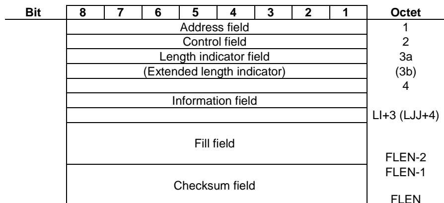
Figure 6.1.1: Frame format type FA
