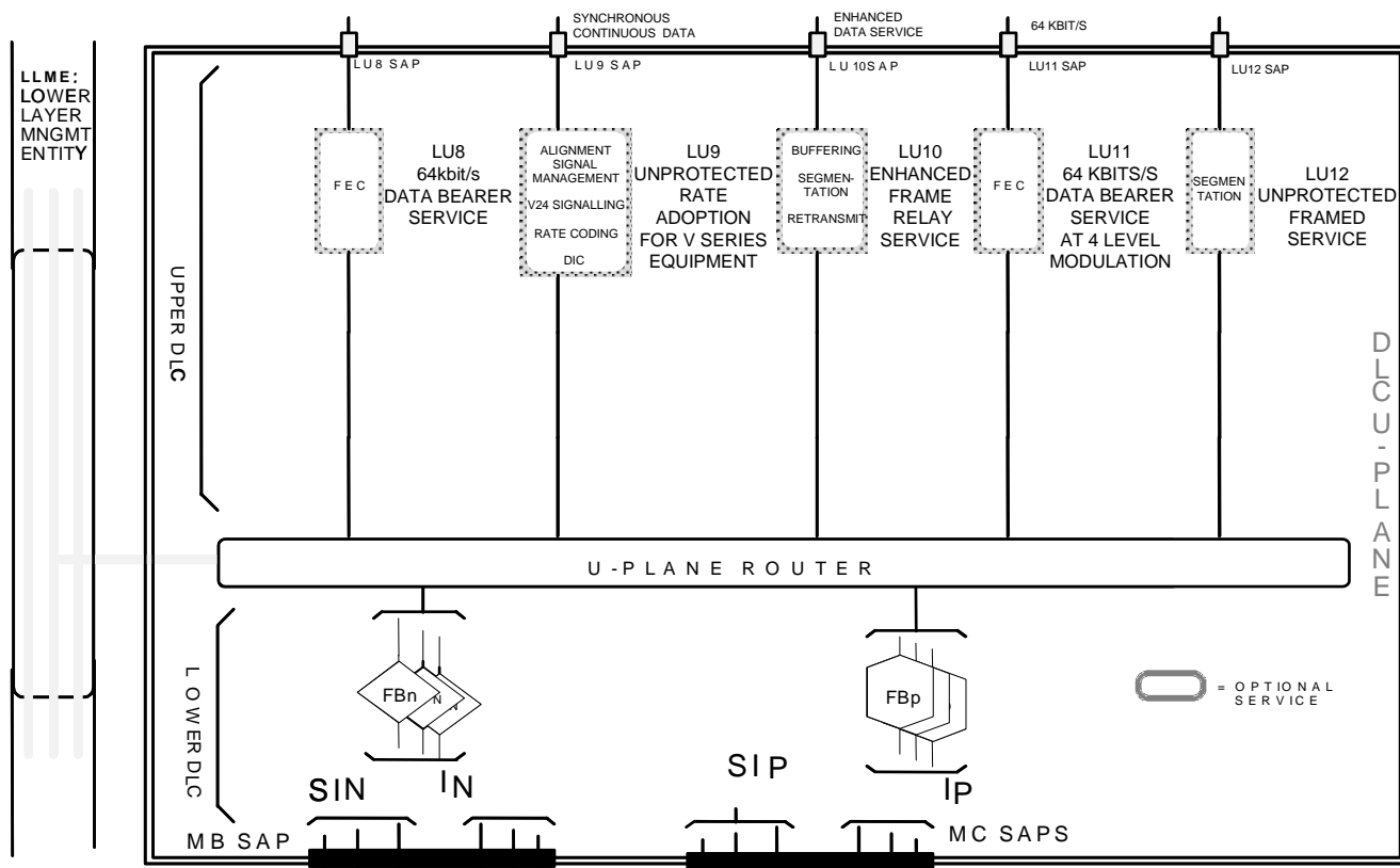
Figure 4.3.1: U-plane model
