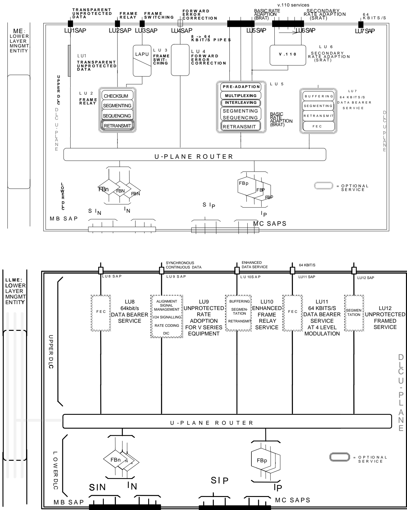
Figure 4.3.1: U-plane model
