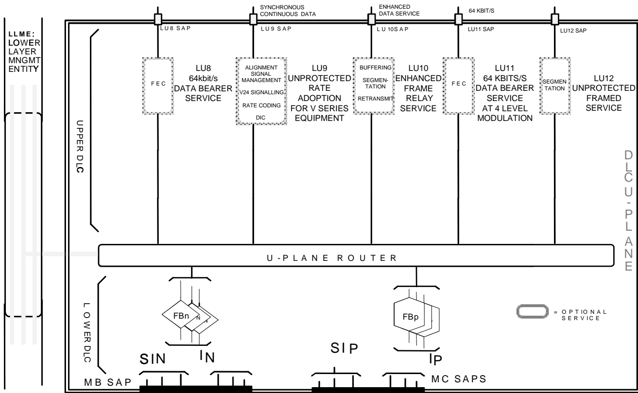
Figure 4.3.1: U-plane model
