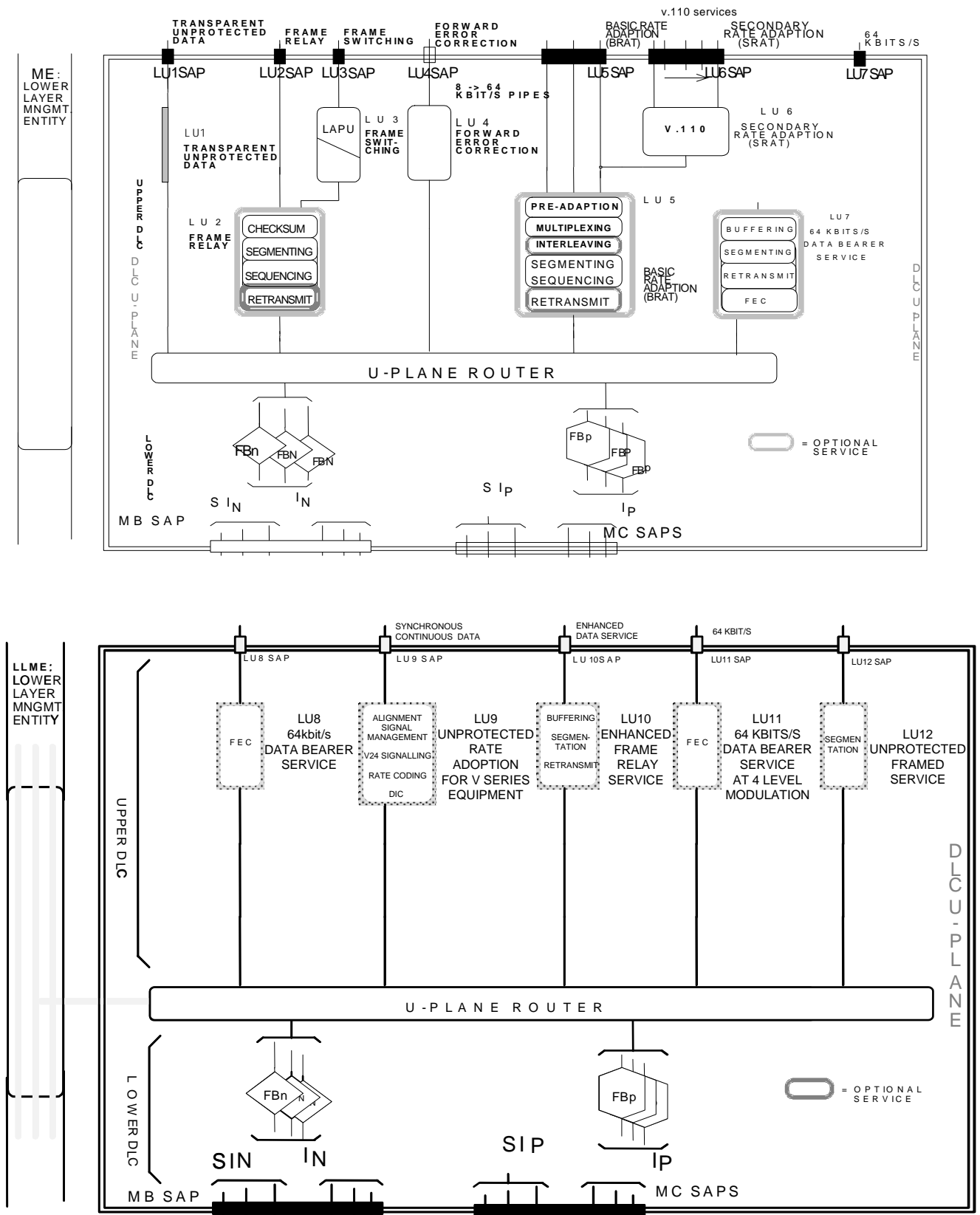
Figure 4.3.1: U-plane model
