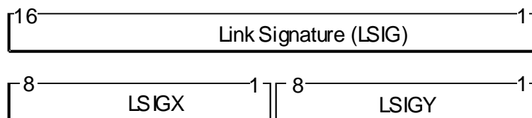
Figure 7.10.1: Link signature
