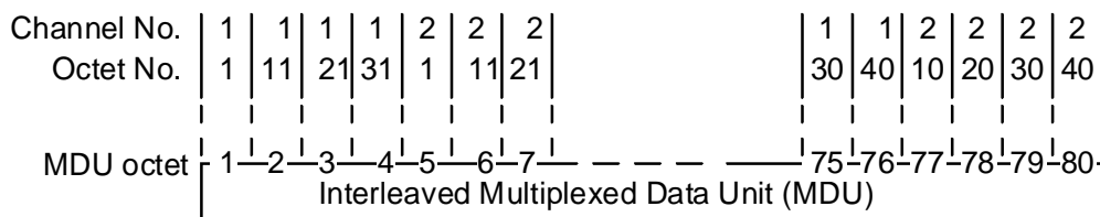
Figure 11.6.3.3.2: Example of interleaved packing (MCS Ref: N2/32)
