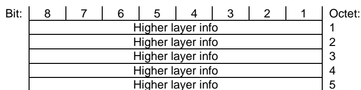
Figure 6.2.1.2: Long frame format (5 octets)
