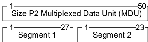
Figure 11.6.2.4.2: Segmentation of Size P2 MDU
