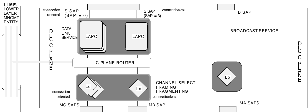
Figure 4.2.1: C-plane model
