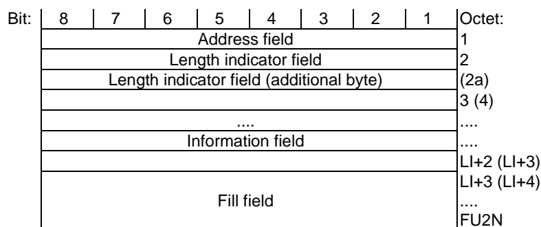
Figure 12.3.1.1: Frame Format Type FU2
