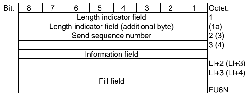
Figure 12.7.1.1: Frame format type FU6a
