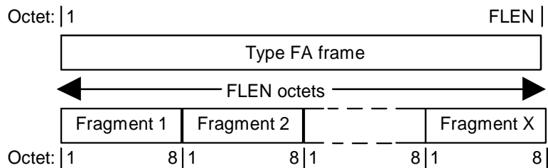
Figure 6.1.4.1.1: C F /CL F logical channel fragmentation
