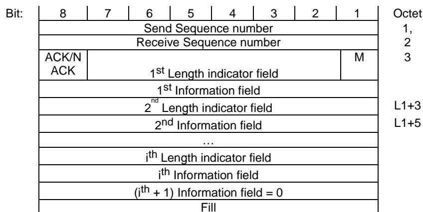
Figure 12.11.1.2: Frame format type FU10b
