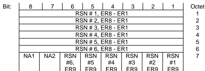
Figure 12.11.1.3: Frame format type FU10c
