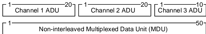
Figure 11.6.2.3.1: Example of non-interleaved packing (MCS Ref: P2/16)
