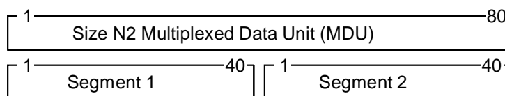
Figure 11.6.3.4.1: Segmentation of Size N2 MDU
