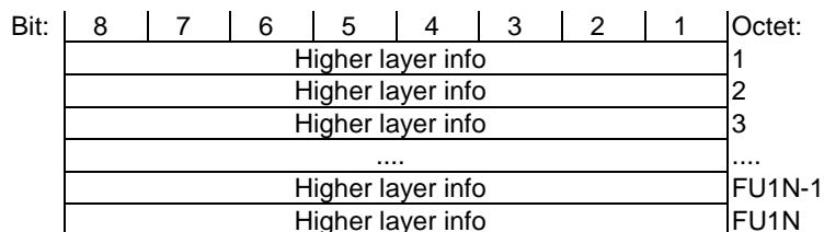
Figure 12.2.1.1: Frame Format Type FU1
