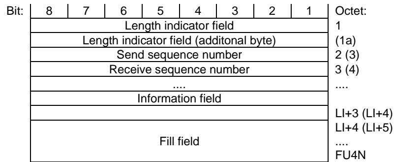
Figure 12.5.1.1: Frame format type FU4a
