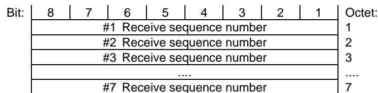
Figure 12.7.1.2: Frame format type FU6b
