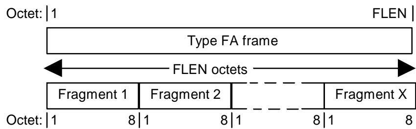
Figure 6.1.4.1.1: C_F/CL_F logical channel fragmentation
