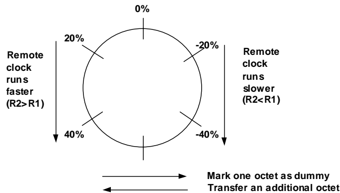
Figure 11.11.5.2.1: Phases diagram
