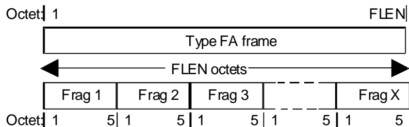
Figure 6.1.4.2.1: C_S/CL_S logical channel fragmentation
