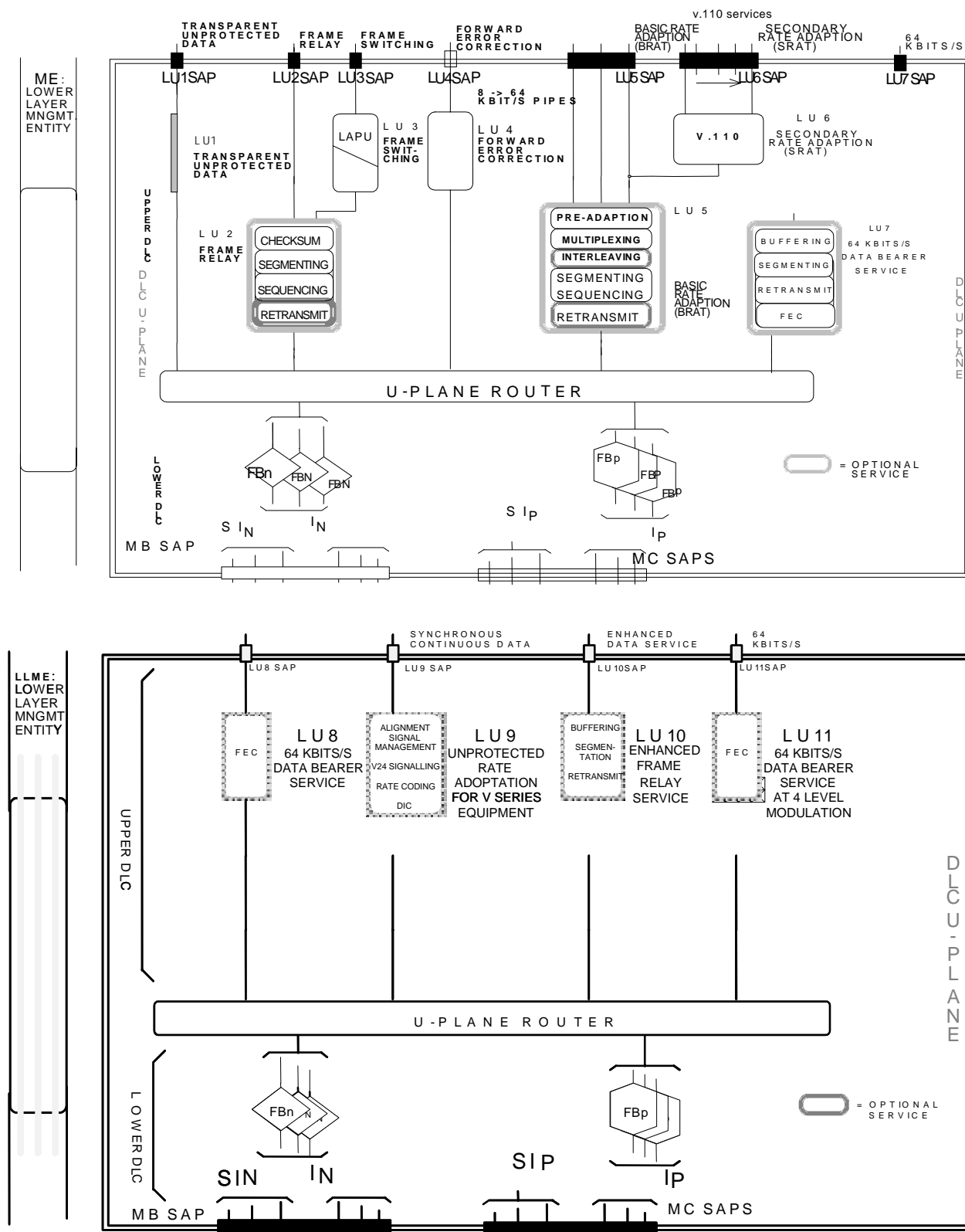
Figure 4.3.1: U-plane model
