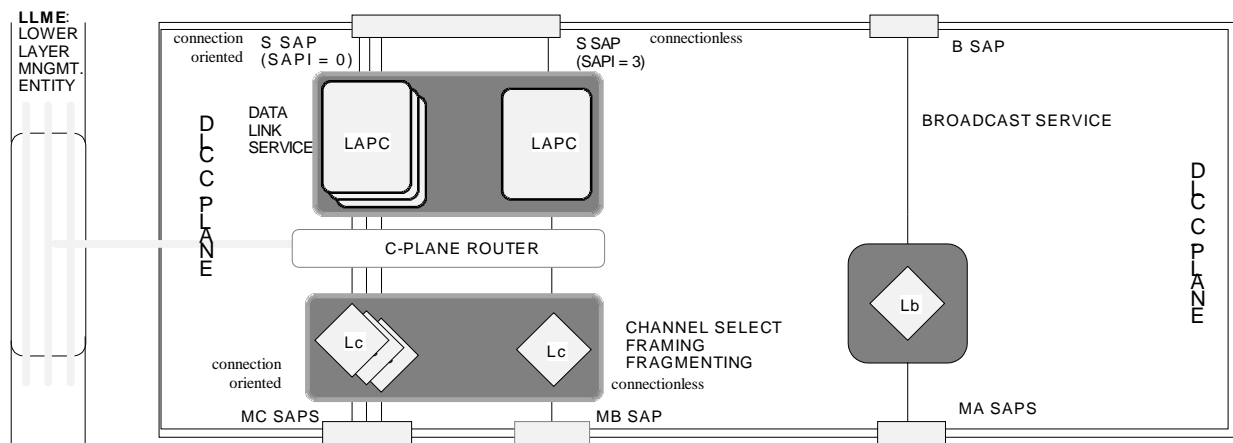
Figure 4.2.1: C-plane model
