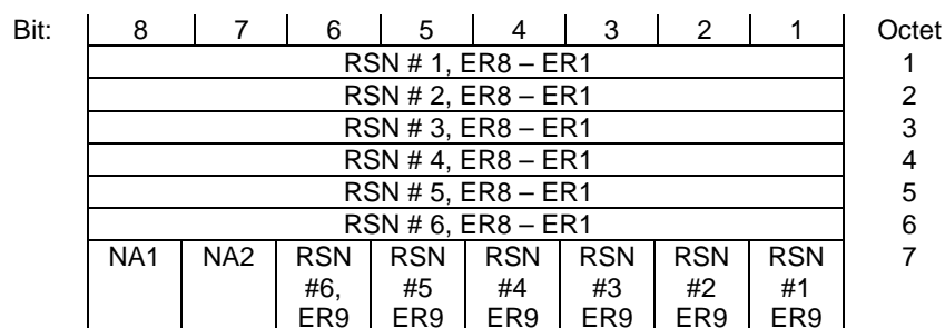
Figure 12.11.1.3: Frame format type FU10c
