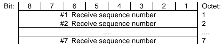
Figure 12.5.1.2: Frame format type FU4b
