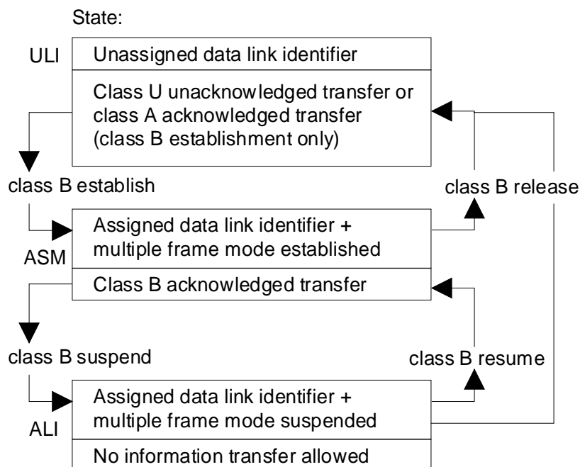
Figure 5.1.3.2.1: LAPC states
