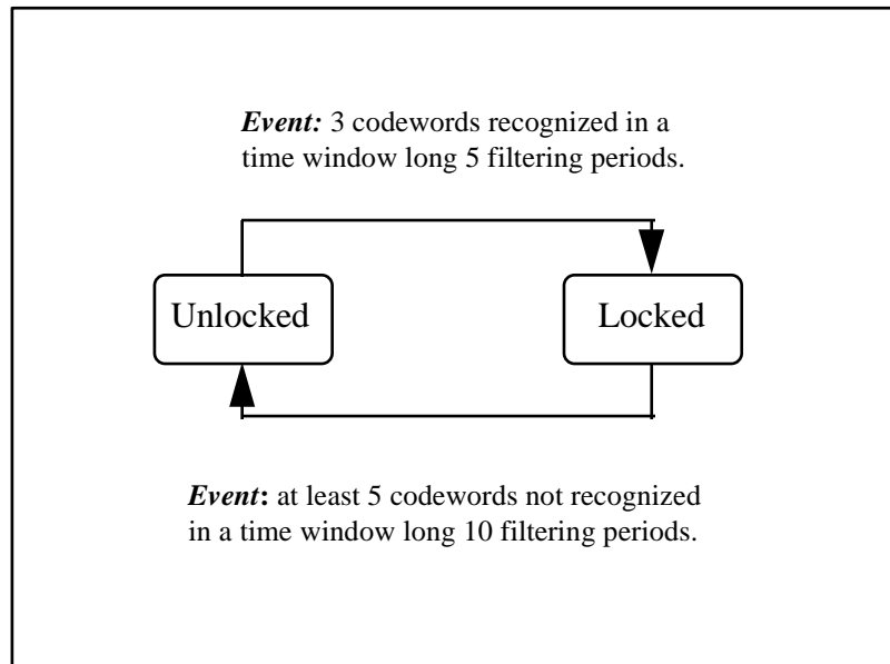
Figure 11.11.2.2.1: Receiver side states
