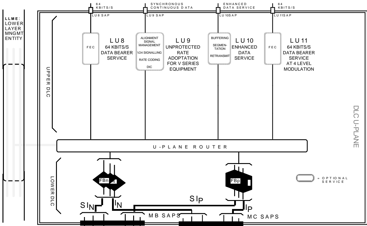
Figure 2: U-plane model
