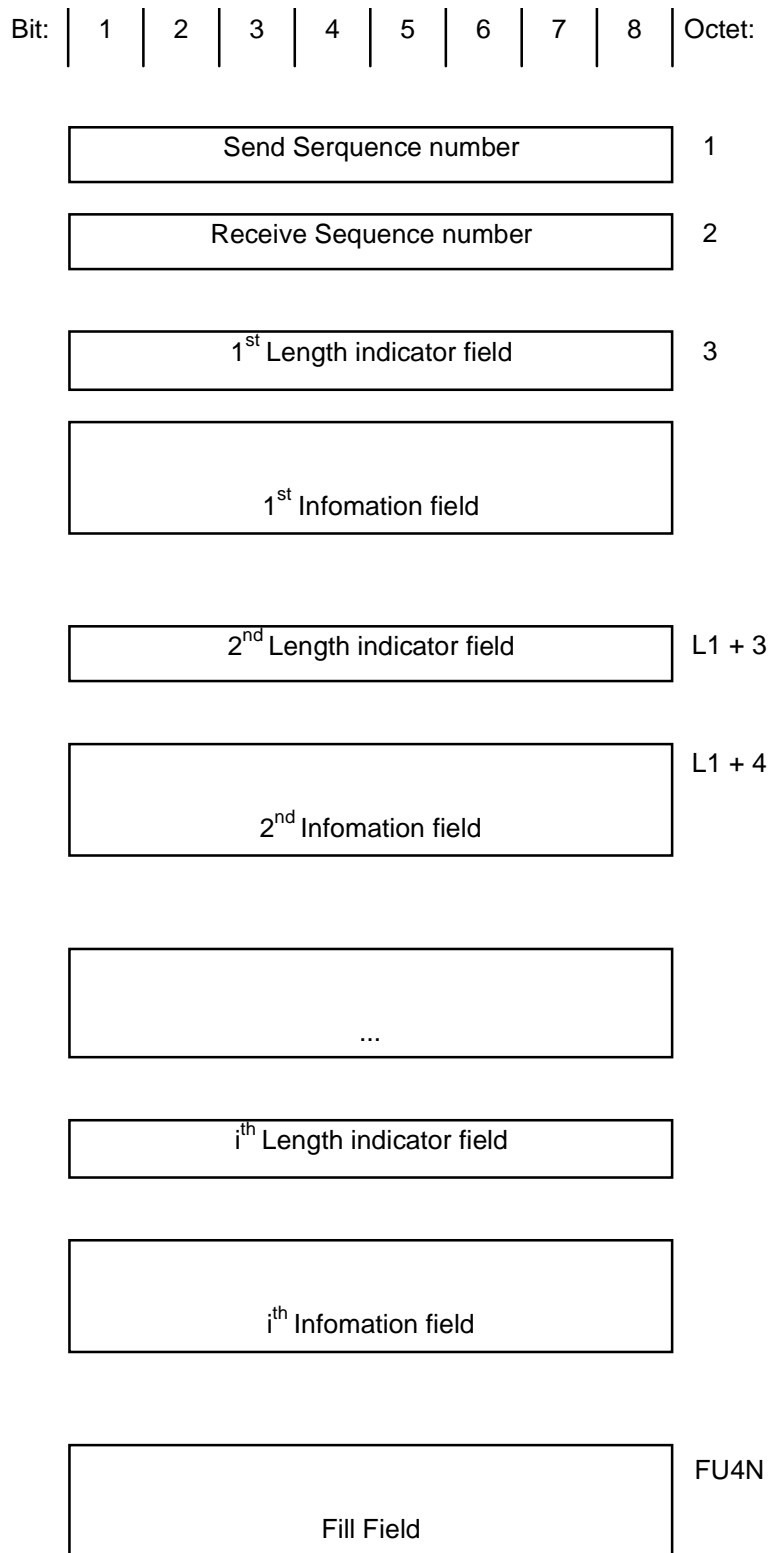
Figure 56: Frame format type FU10b
