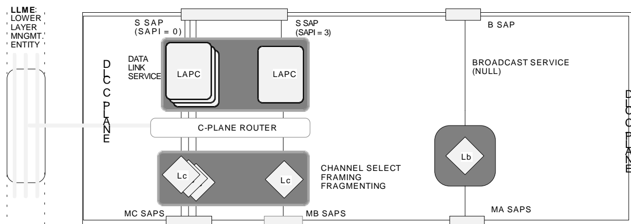
Figure 1: C-plane model
