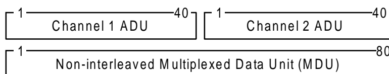
Figure 28: Example of non-interleaved packing (MCS Ref: N2/32)
