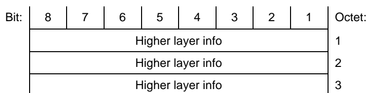
Figure 7: Short frame format (3 octets)
