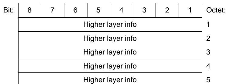
Figure 8: Long frame format (5 octets)
