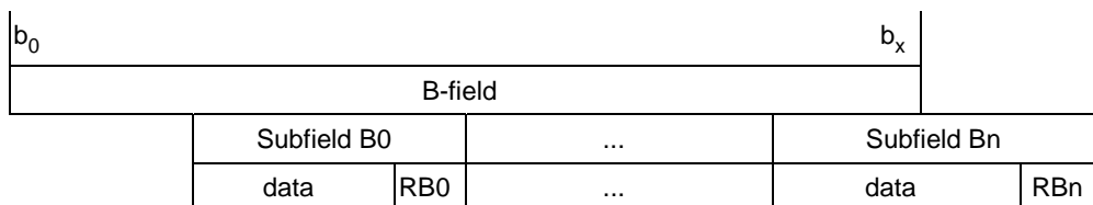
Figure 6.13d: B-field structure of the constant-size subfield protected format for any other higher level modulation
