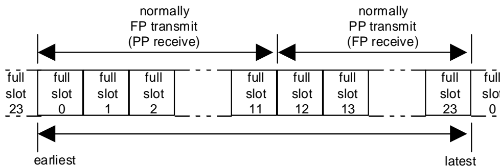
Figure 4.3: Full Slots
