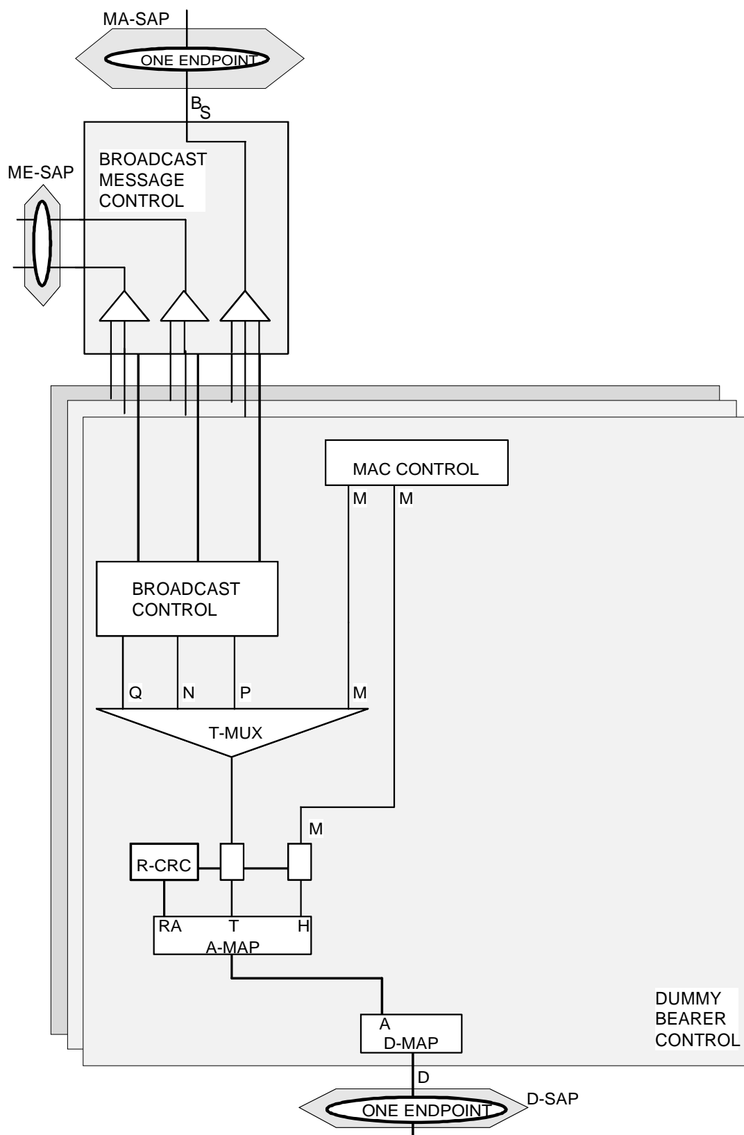
Figure 6.3: DBC multiplexing
