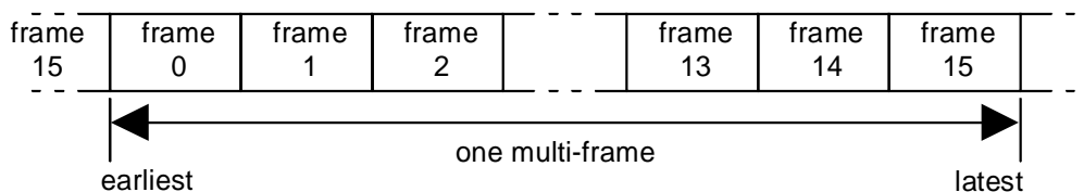
Figure 4.6: Multiframe
