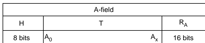
Figure 6.10: A-field mapping
