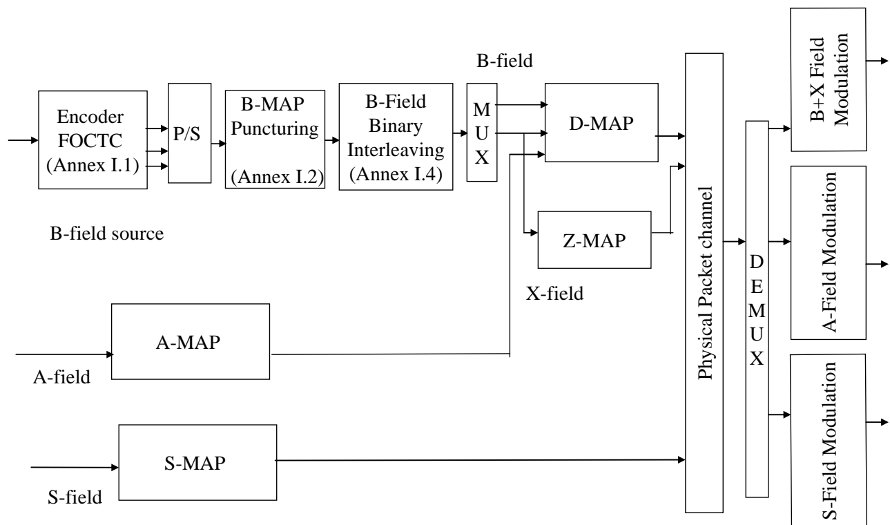
Figure I.1: B-field Channel Encoding scheme
