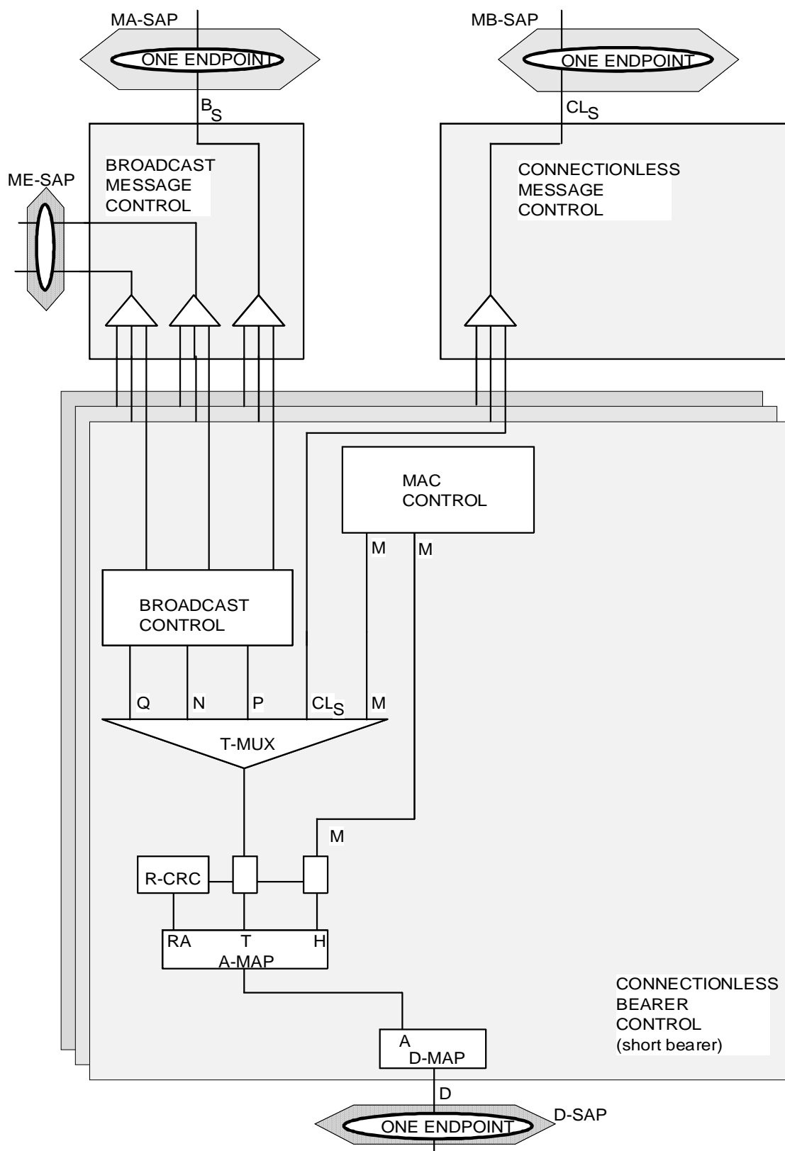
Figure 6.4: CBC multiplexing (short)
