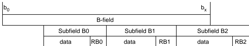
Figure 6.13c: B-field structure of the constant-size subfield protected format for 8-level modulation
