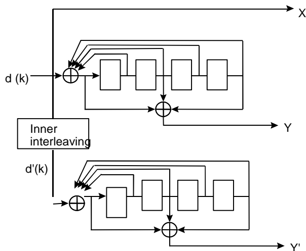
Figure I.4: FOCTC structure
