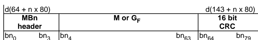
Figure 7.65: B-field messages
