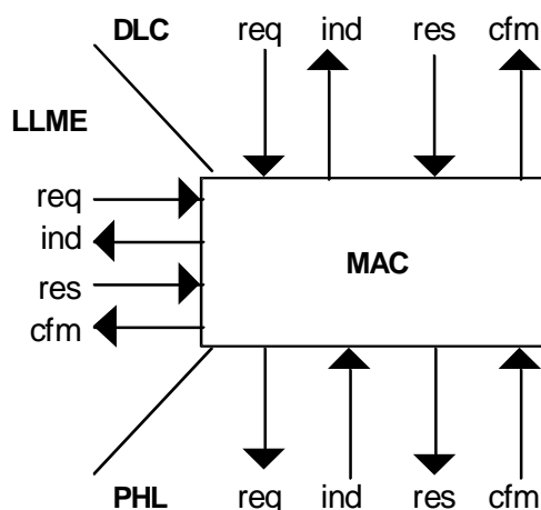
Figure 8.1: MAC layer primitives
