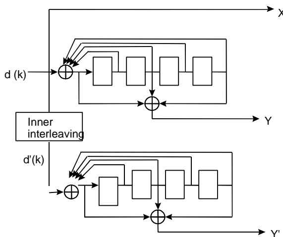
Figure I.4: FOCTC structure
