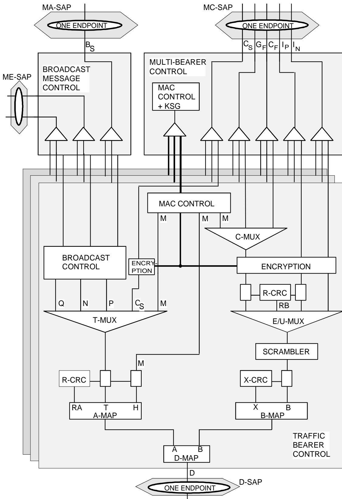
Figure 6.1: TBC multiplexing
