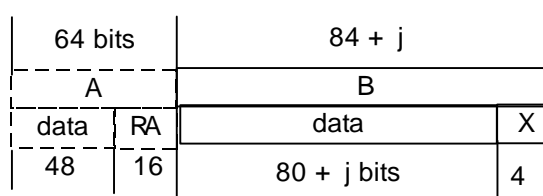
Figure 6.22: Unprotected D08 B-field format (half slot, 2 level modulation)
