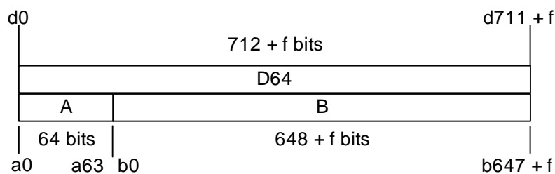
Figure 6.9: A-field and B-field in the D64 field (full slot, 4 level modulation)
