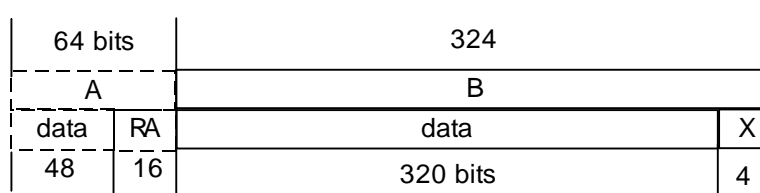
Figure 6.19: Unprotected D32 B-field format (full slot, 2 level modulation)
