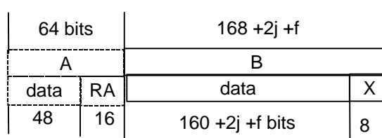
Figure 6.23: Unprotected D16 B-field format (half slot, 4 level modulation)
