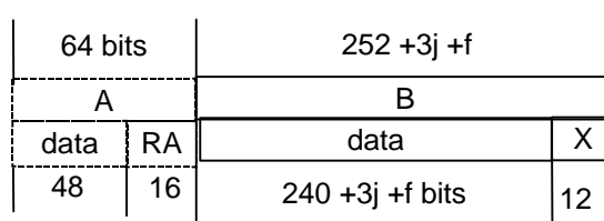
Figure 6.24: Unprotected D24 B-field format (half slot, 8 level modulation)
