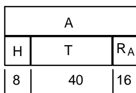
Figure 6.15: A-field mapping
