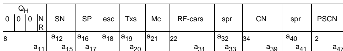
Figure 7.6: Static System Information
