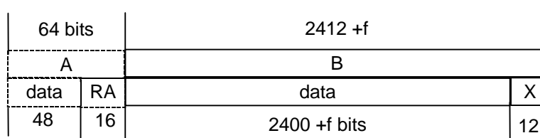
Figure 6.18: Unprotected D240 B-field format (double slot, 8 level modulation)
