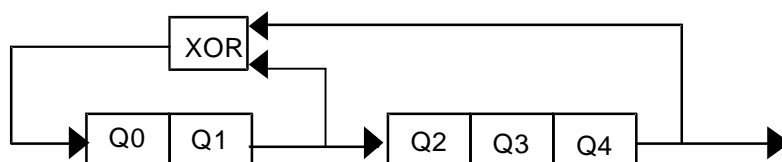
Figure 6.40: Scrambling sequence generation
