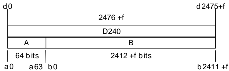
Figure 6.7: A-field and B-field in the D240 field (double slot, 8 level modulation)
