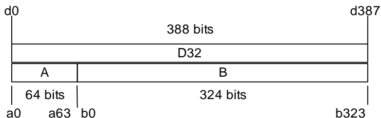
Figure 6.8: A-field and B-field in the D32 field (full slot, 2 level modulation)
