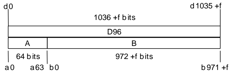
Figure 6.10: A-field and B-field in the D96 field (full slot, 8 level modulation)
