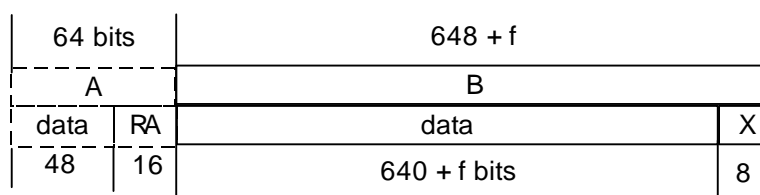
Figure 6.20: Unprotected D64 B-field format (full slot, 4 level modulation)
