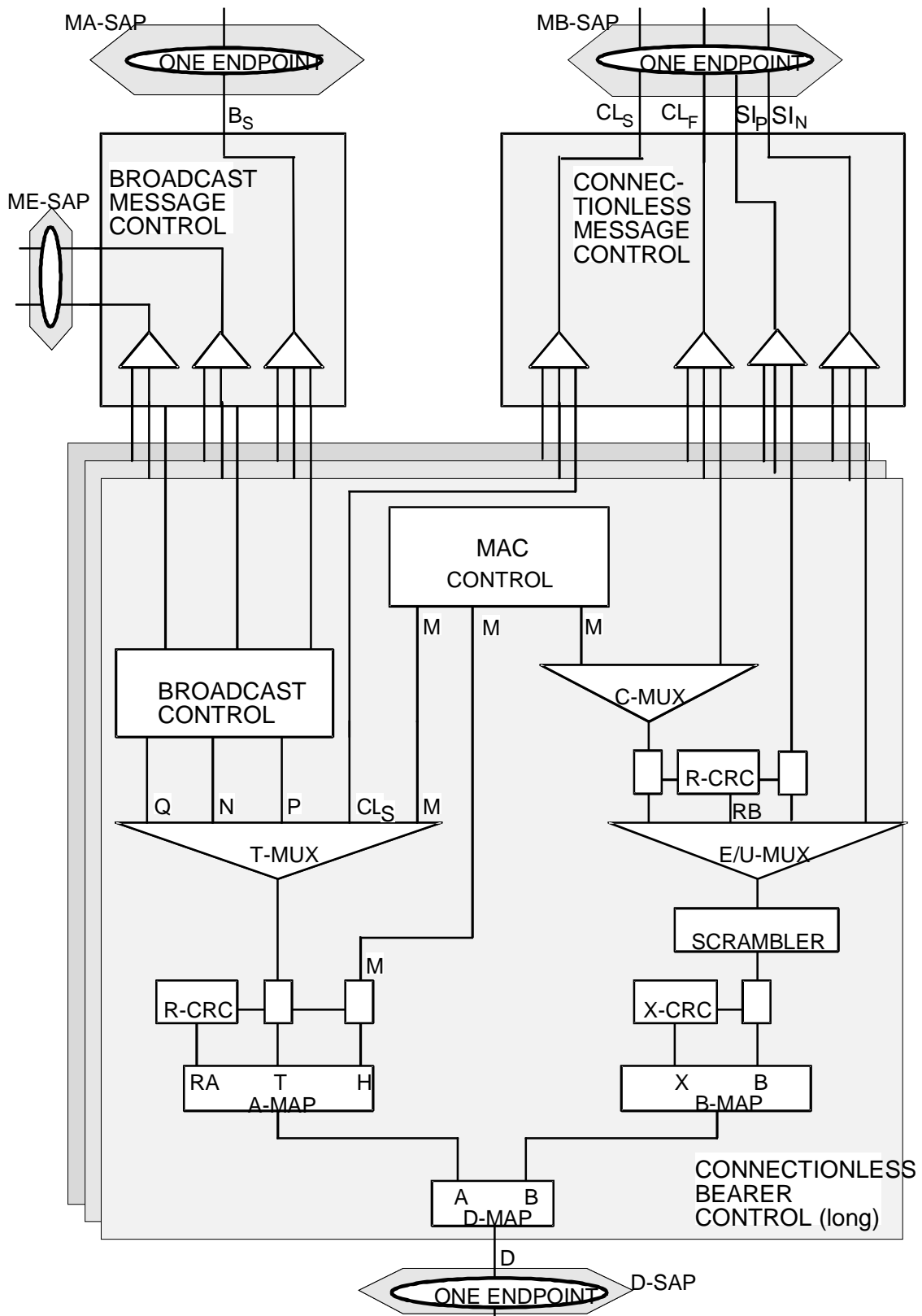
Figure 6.2: CBC multiplexing (long)
