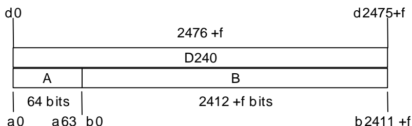
Figure 6.7: A-field and B-field in the D240 field (double slot, 8 level modulation)
