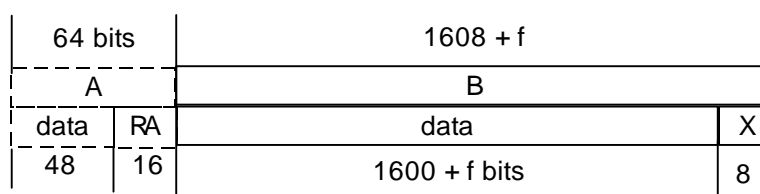
Figure 6.17: Unprotected D160 B-field format (double slot, 4 level modulation)
