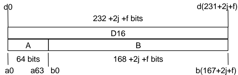
Figure 6.12: A-field and B-field in the D16 field (half slot, 4 level modulation)
