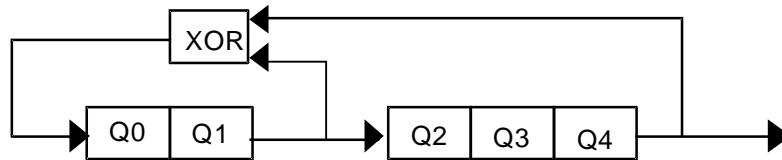
Figure 6.40: Scrambling sequence generation
