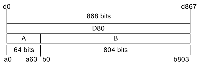
Figure 6.5: A-field and B-field in the D80 field (double slot, 2 level modulation)
