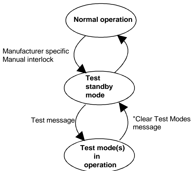
Figure 12.1: State mode diagram for IUTs during testing
