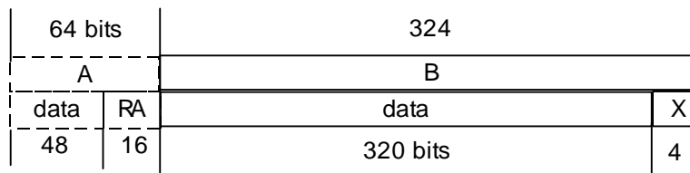
Figure 6.19: Unprotected D32 B-field format (full slot, 2 level modulation)
