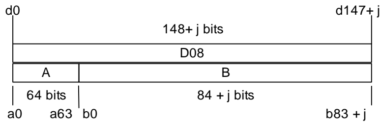
Figure 6.11: A-field and B-field in the D08 field (half slot, 2 level modulation)
