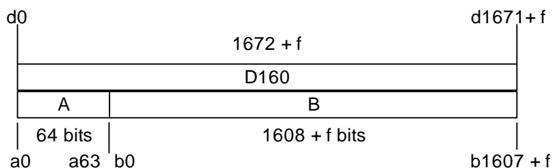
Figure 6.6: A-field and B-field in the D160 field (double slot, 4 level modulation)
