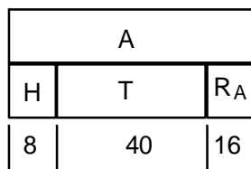
Figure 6.15: A-field mapping
