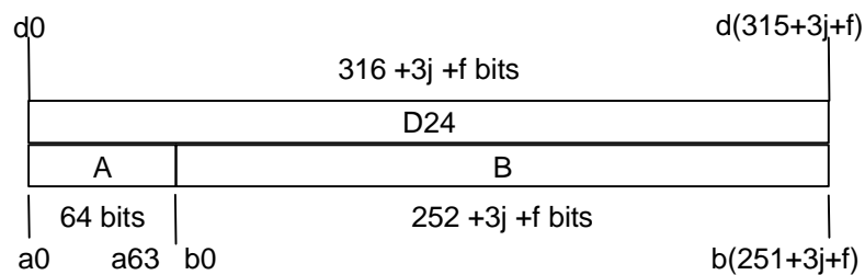
Figure 6.13: A-field and B-field in the D24 field (half slot, 8 level modulation)
