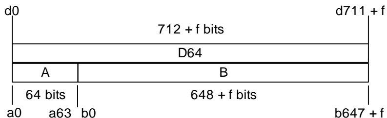
Figure 6.9: A-field and B-field in the D64 field (full slot, 4 level modulation)
