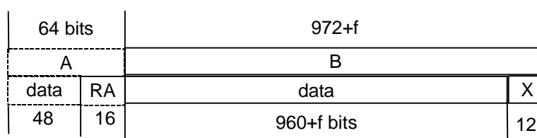
Figure 6.21: Unprotected D96-field format (full slot, 8 level modulation)
