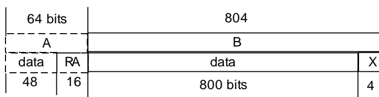
Figure 6.16: Unprotected D80 B-field format (double slot, 2 level modulation)
