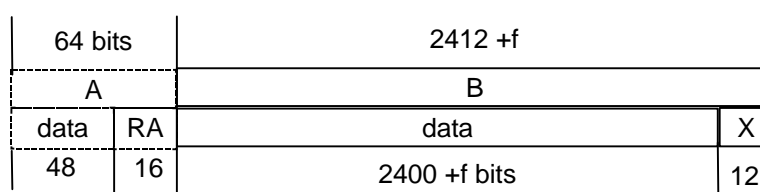
Figure 6.18: Unprotected D240 B-field format (double slot, 8 level modulation)
