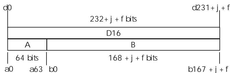
Figure 15b: A-field and B-field in the D16 field (half slot, 4 level modulation)
