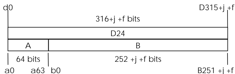
Figure 15c: A-field and B-field in the D24 field (half slot, 8 level modulation)
