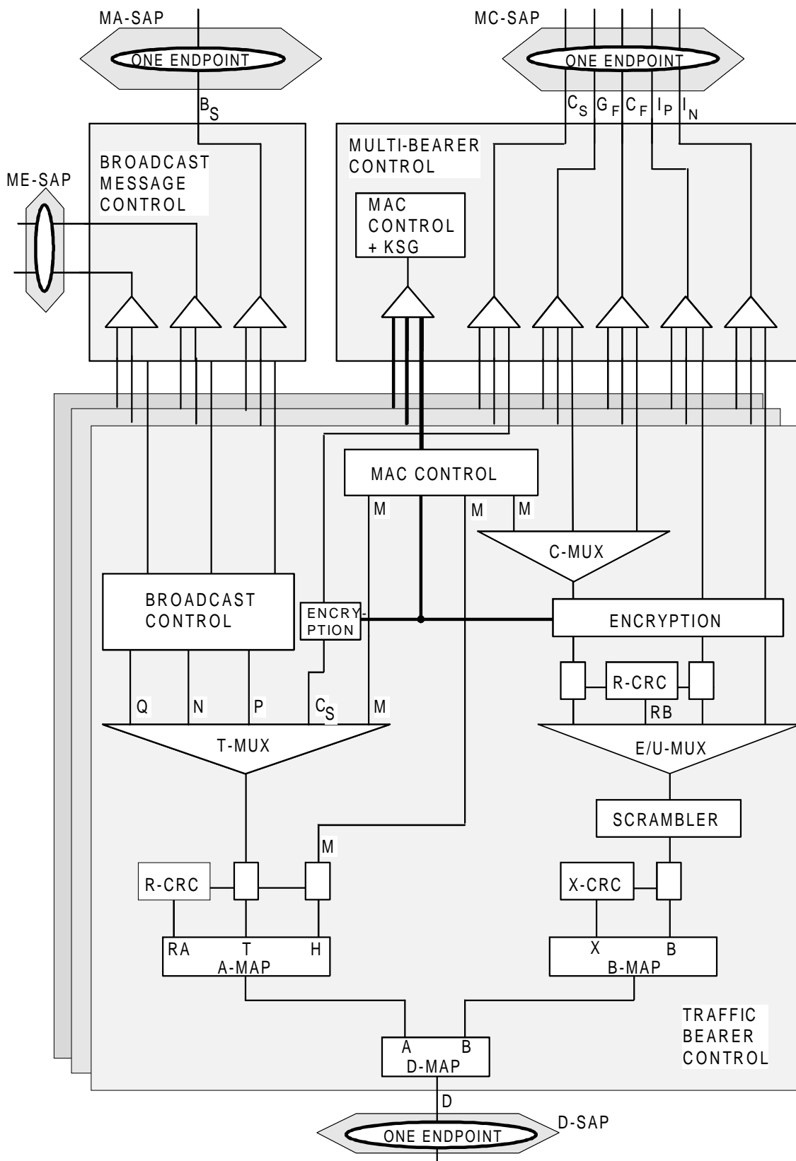
Figure 9: TBC multiplexing
