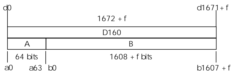
Figure 13b: A-field and B-field in the D160 field (double slot, 4 level modulation)
