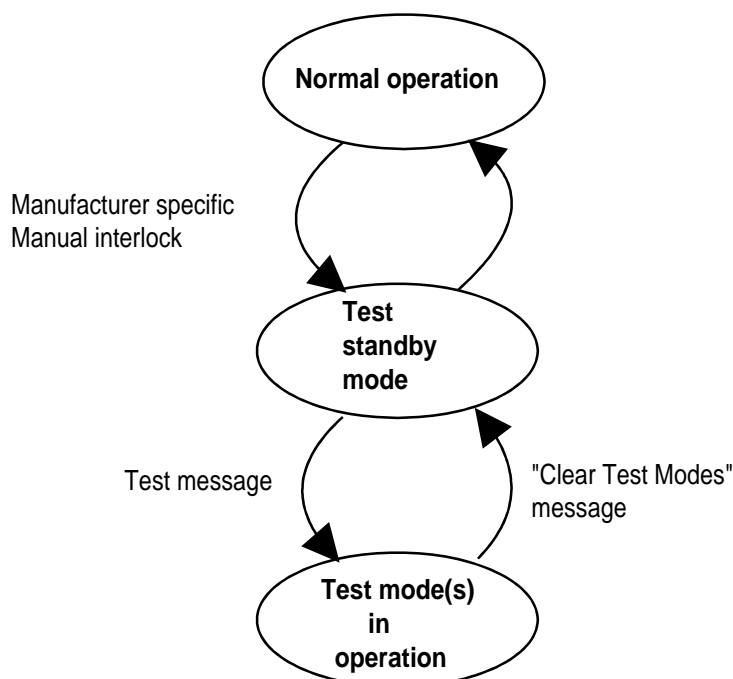
Figure 114: State mode diagram for IUTs during testing
