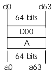
Figure 16: The D00 field containing the A-field
