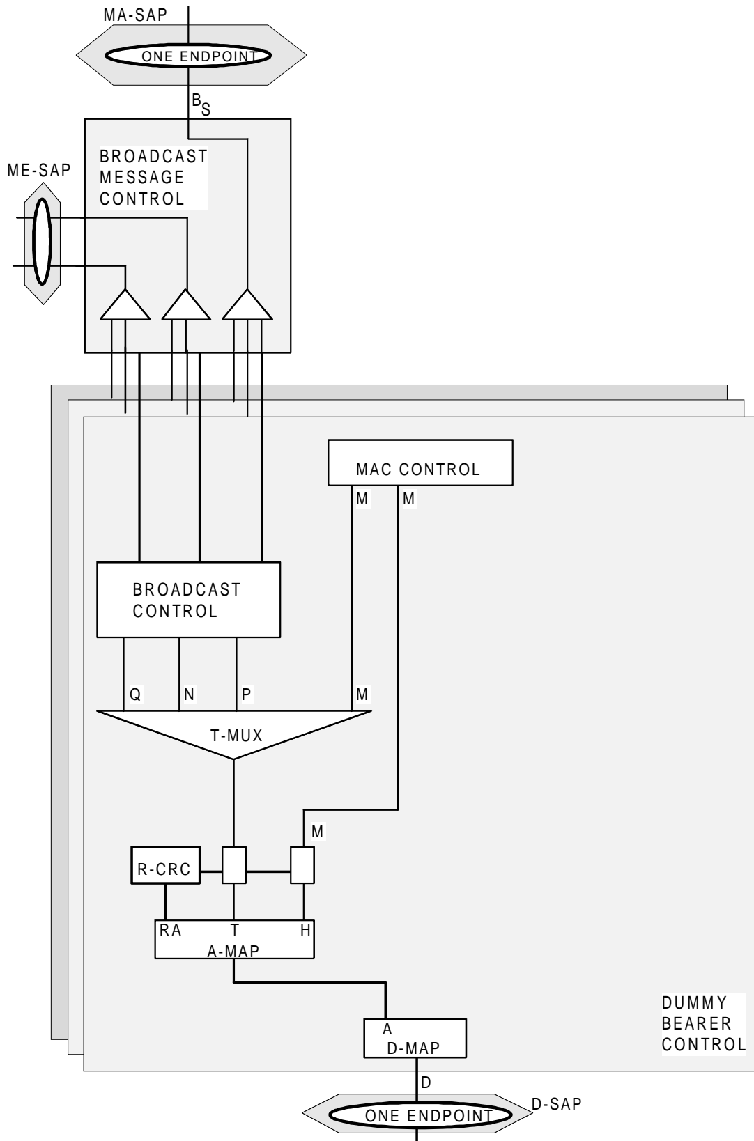
Figure 11: DBC multiplexing
