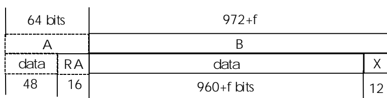
Figure 19c: Unprotected D96-field format (full slot, 8 level modulation)
