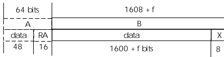
Figure 18b: Unprotected D160 B-field format (double slot, 4 level modulation)
