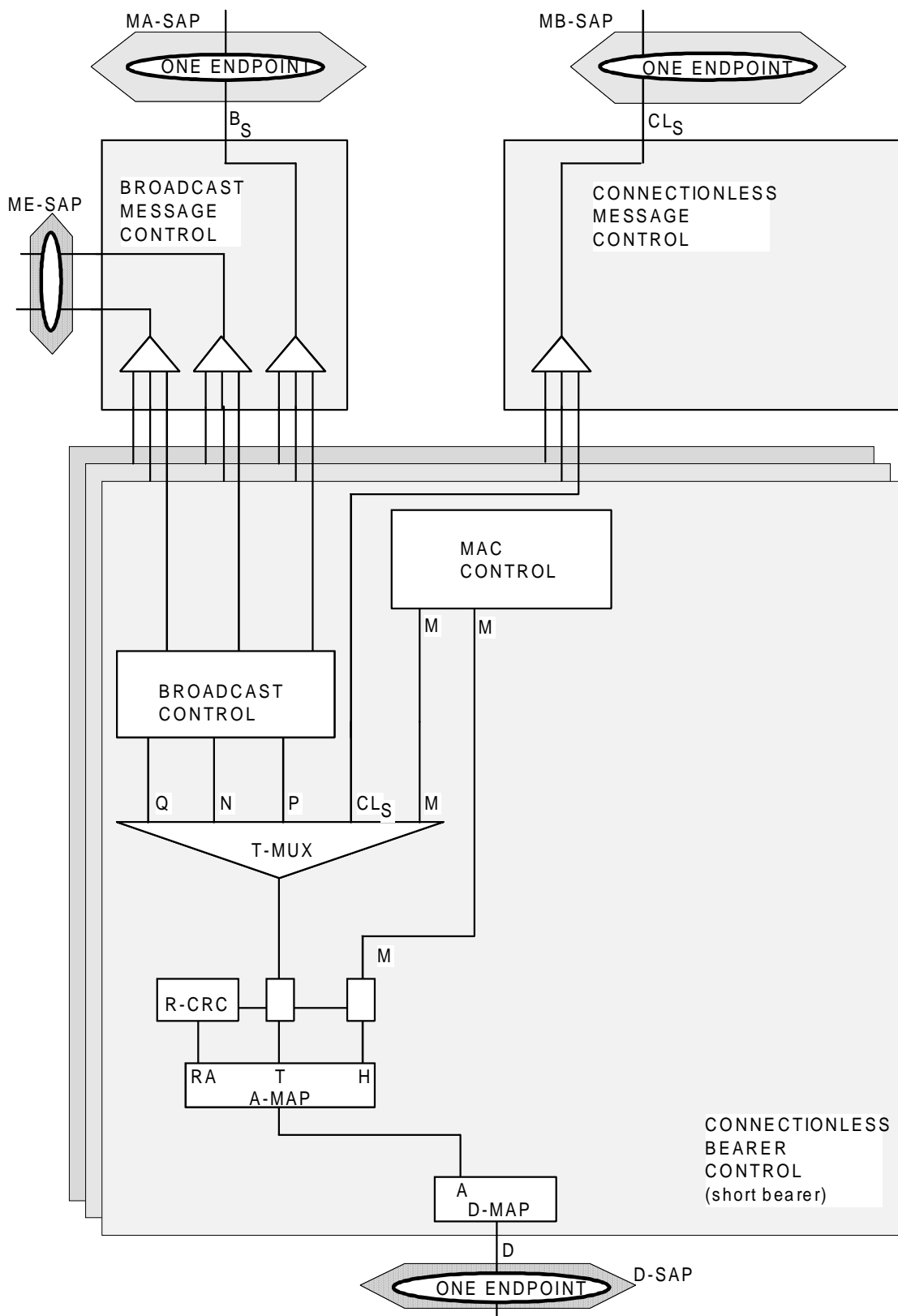
Figure 12: CBC multiplexing (short)
