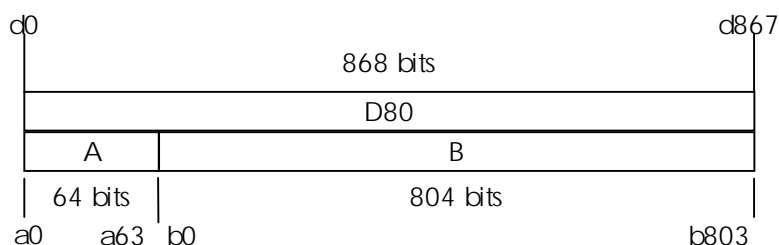
Figure 13a: A-field and B-field in the D80 field (double slot, 2 level modulation)
