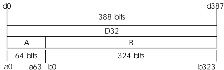
Figure 14a: A-field and B-field in the D32 field (full slot, 2 level modulation)
