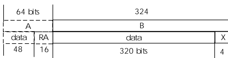
Figure 19a: Unprotected D32 B-field format (full slot, 2 level modulation)
