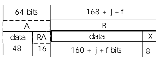
Figure 20b: Unprotected D16 B-field format (half slot, 4 level modulation)
