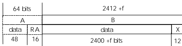
Figure 18c: Unprotected D240 B-field format (double slot, 8 level modulation)
