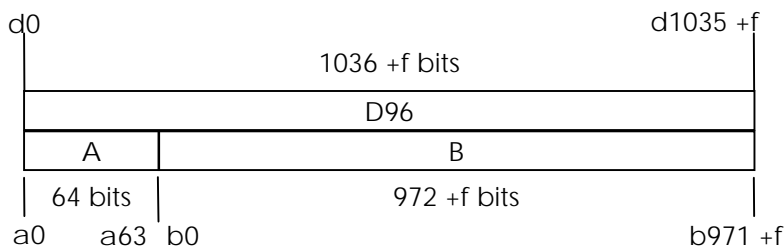
Figure 14c: A-field and B-field in the D96 field (full slot, 8 level modulation)
