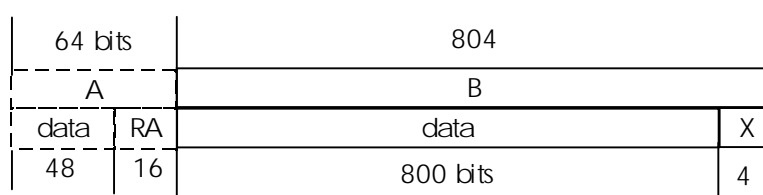
Figure 18a: Unprotected D80 B-field format (double slot, 2 level modulation)
