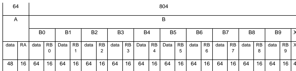
Figure 21a: Protected B-field format D80 (double slot, 2 level modulation)
