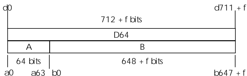
Figure 14b: A-field and B-field in the D64 field (full slot, 4 level modulation)
