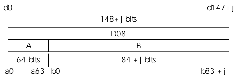
Figure 15a: A-field and B-field in the D08 field (half slot, 2 level modulation)
