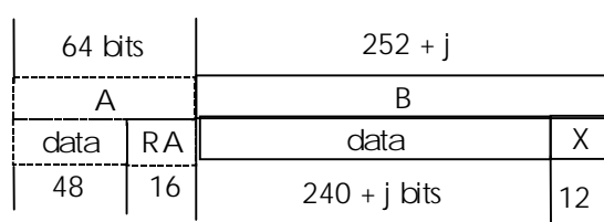
Figure 20c: Unprotected D24 B-field format (half slot, 8 level modulation)
