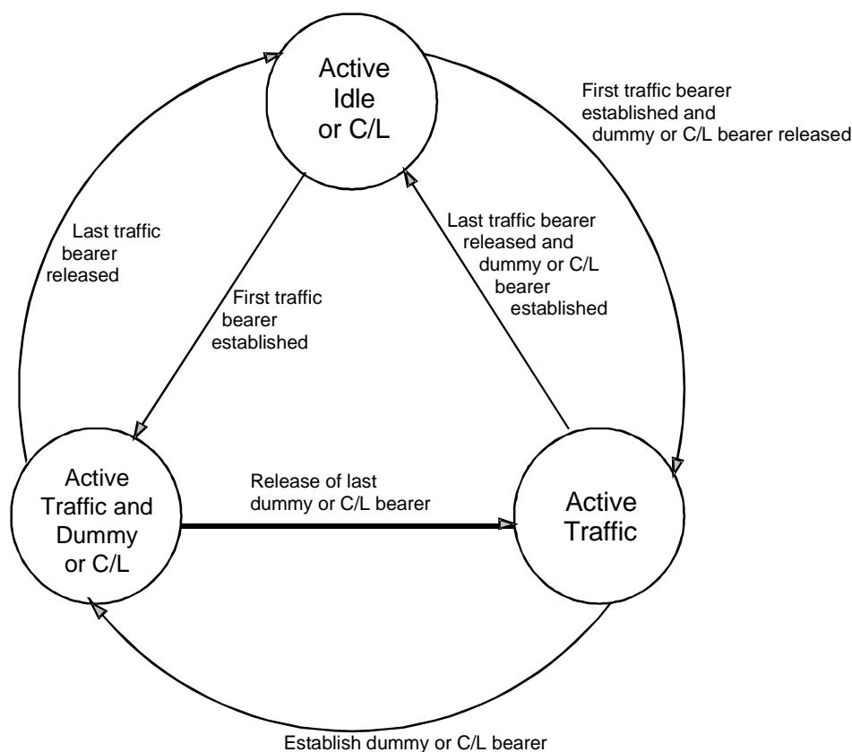
Figure 8: RFP state diagram
