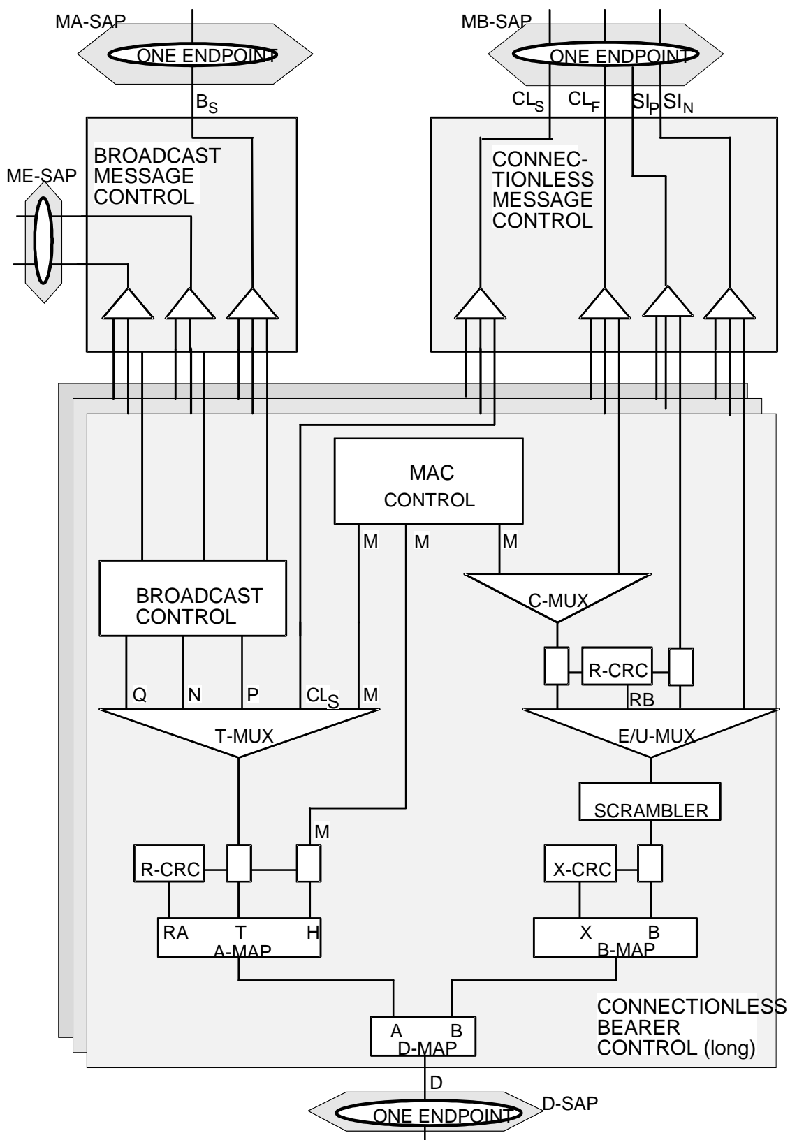
Figure 10: CBC multiplexing (long)
