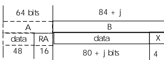
Figure 20a: Unprotected D08 B-field format (half slot, 2 level modulation)
