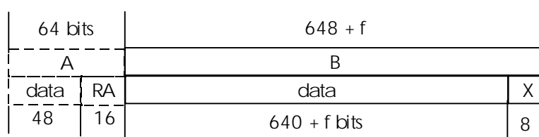
Figure 19b: Unprotected D64 B-field format (full slot, 4 level modulation)
