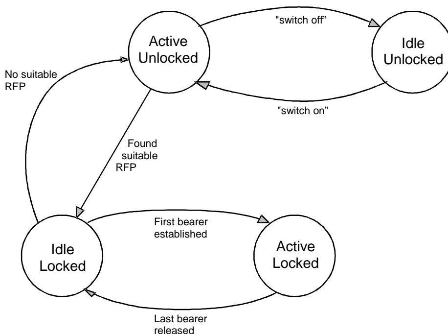
Figure 7: PP state diagram
