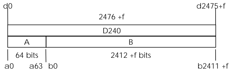
Figure 13c: A-field and B-field in the D240 field (double slot, 8 level modulation)
