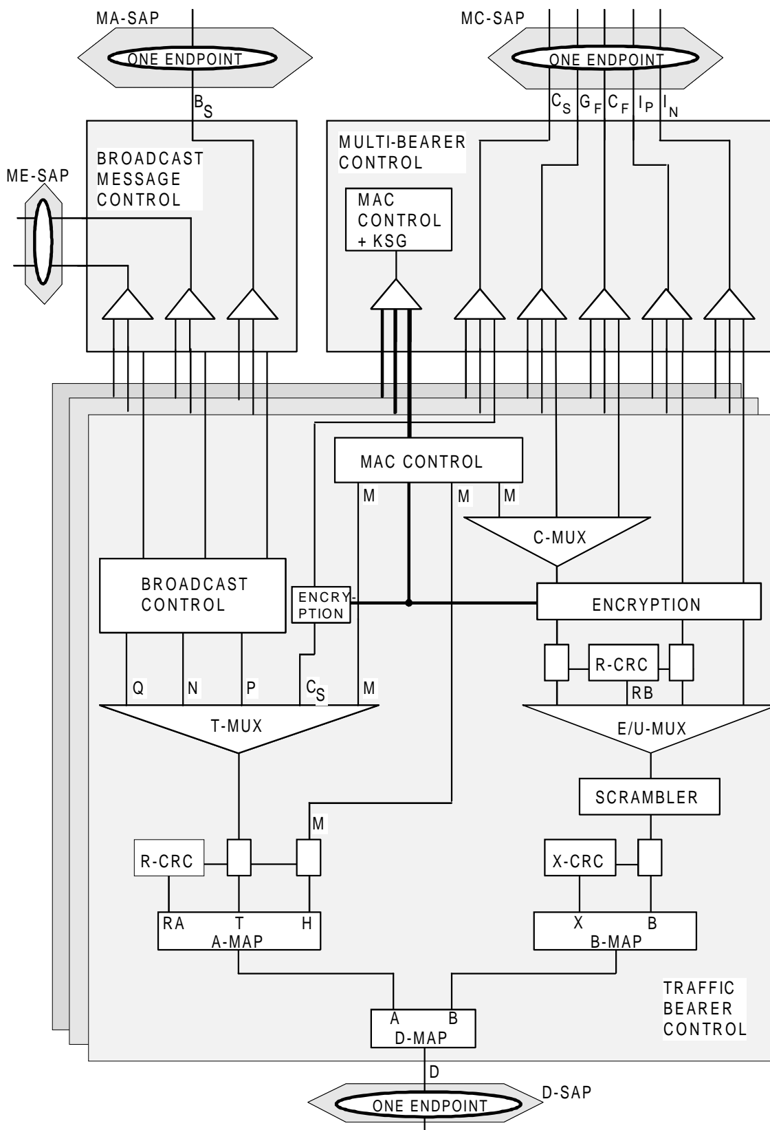
Figure 9: TBC multiplexing
