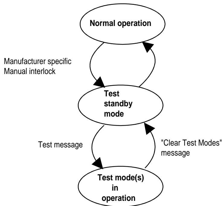
Figure 111: State mode diagram for IUTs during testing
