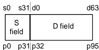
Figure 14: P00 packet
