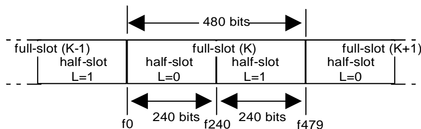
Figure 2: Half-slot format
