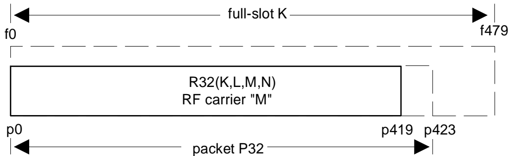
Figure 10: Basic physical channel R32
