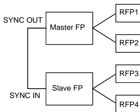
Figure B.1: Synchronization ports configuration
