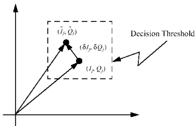
Figure D.3: Error vector calculation
