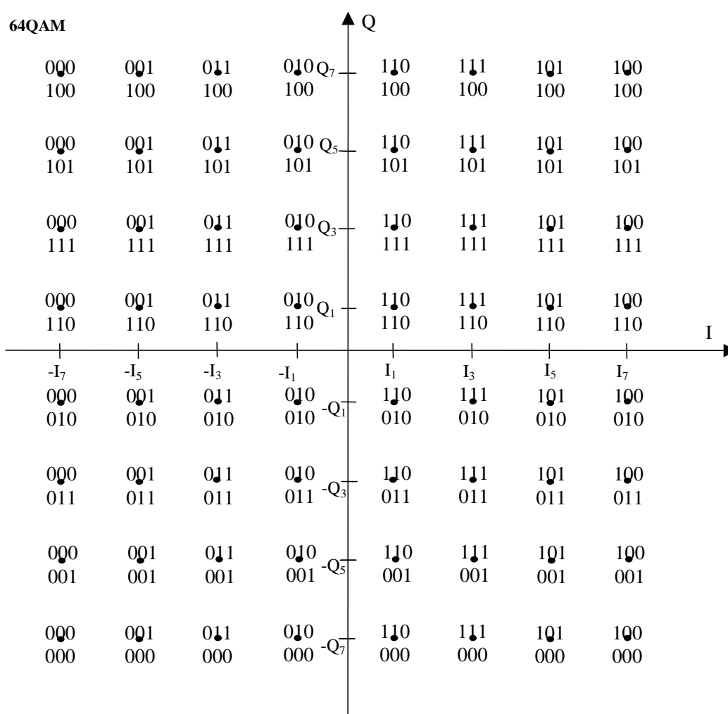
Figure D.2: 64 QAM constellation
