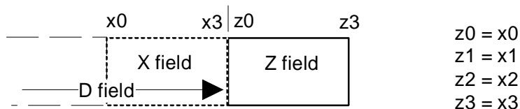
Figure 16: The Z-field
