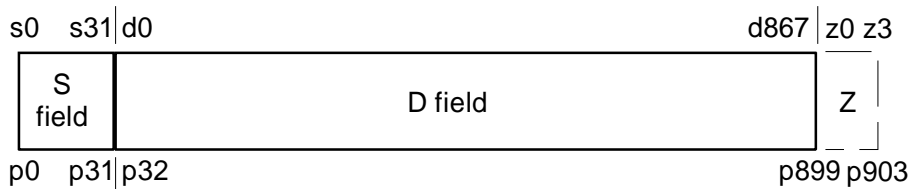
Figure 15: Packet P80
