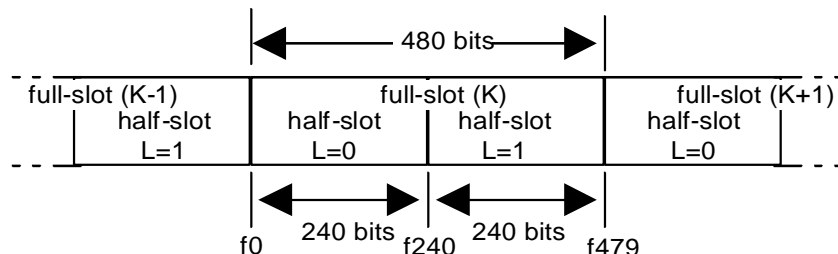
Figure 2: Half-slot format
