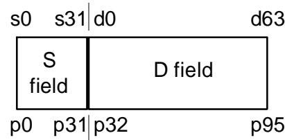
Figure 12: P00 packet
