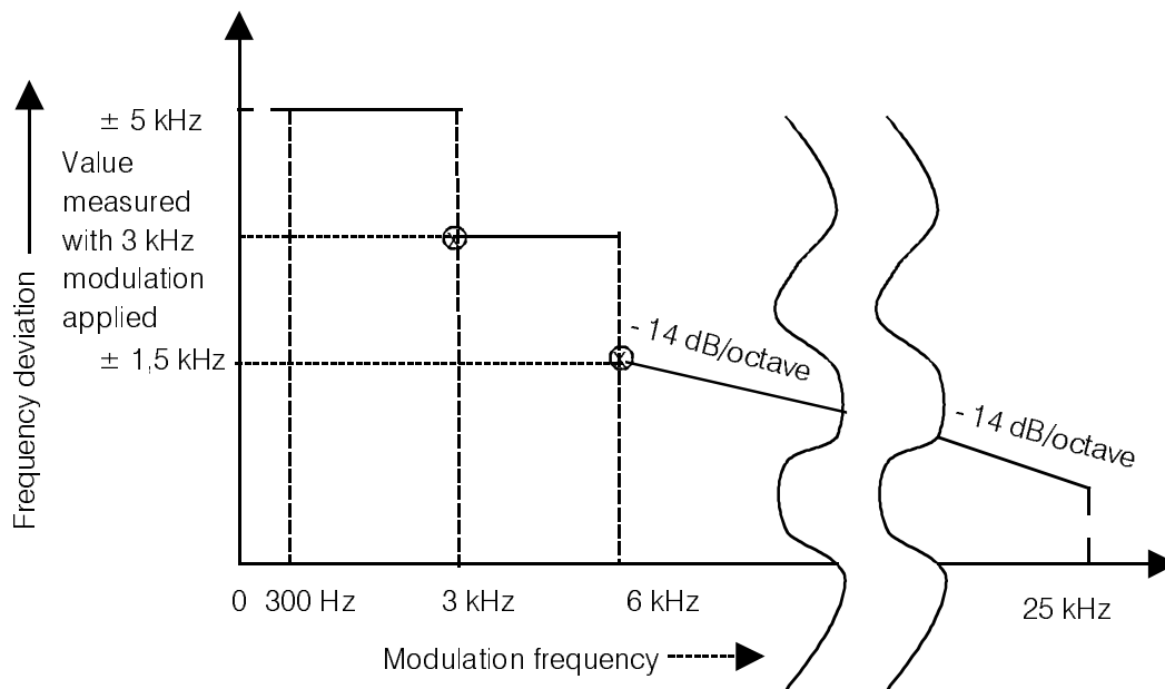
Figure 1: Frequency deviation
