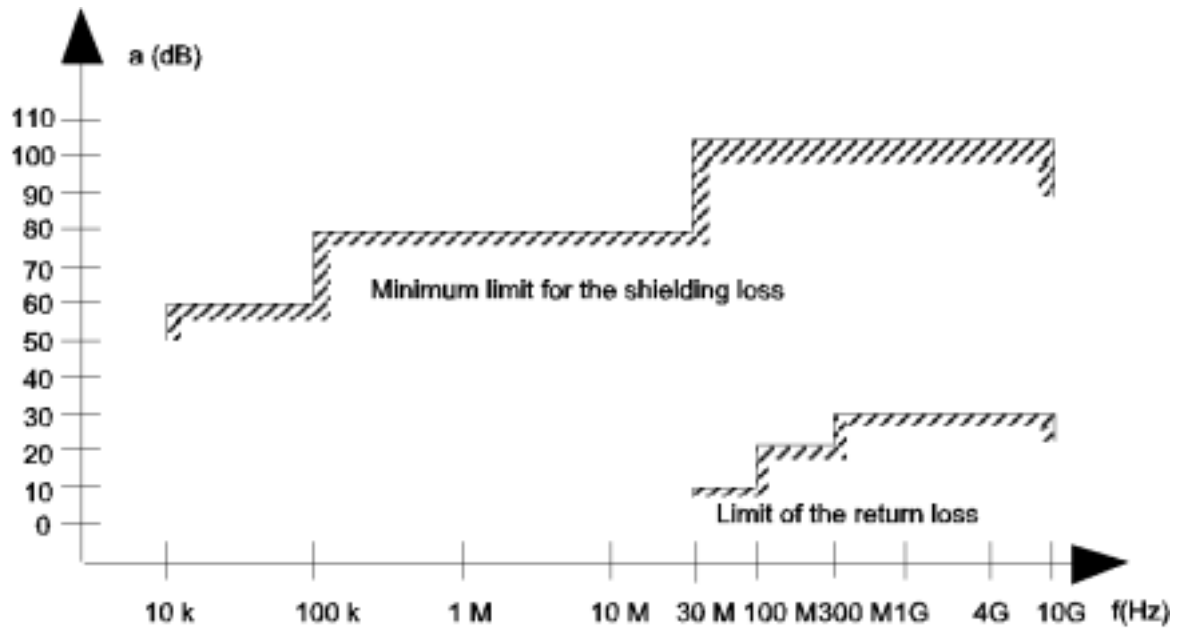
Figure C.3: Specifications for shielding and reflections
