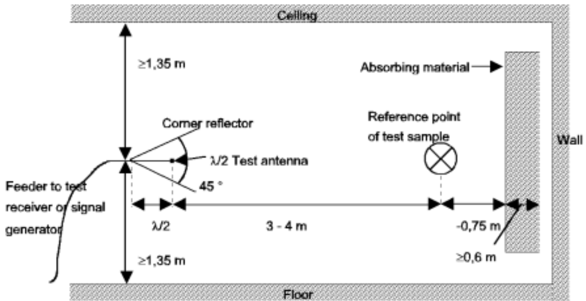
Figure C.2: Indoor site arrangement (shown for horizontal polarization)
