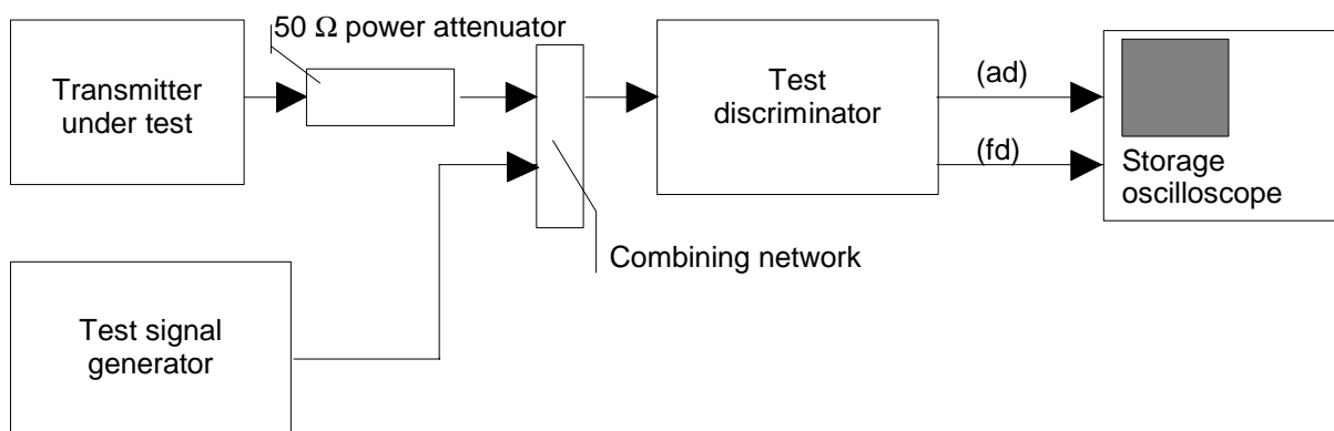
Figure 5: Measurement arrangement
