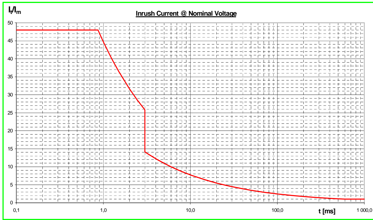
Figure 2: Maximum inrush current ratio characteristics for equipment at nominal voltage and maximum load
