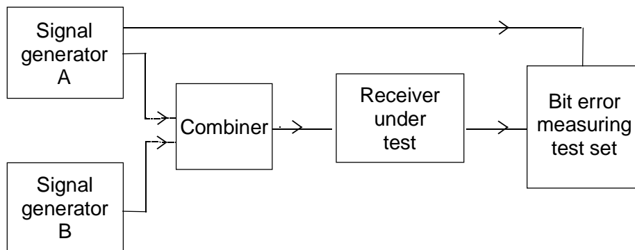
Figure 22: Measurement arrangement
