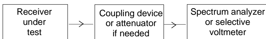
Figure 31: Measurement arrangement
