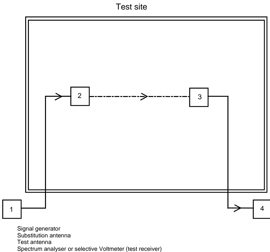
Figure 11: Measurement arrangement
