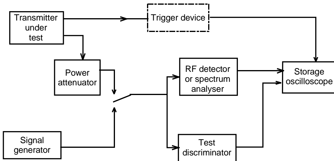
Figure 16: Test arrangement for transient behaviour of transmitter power and frequency, including transmitter attack and release time
