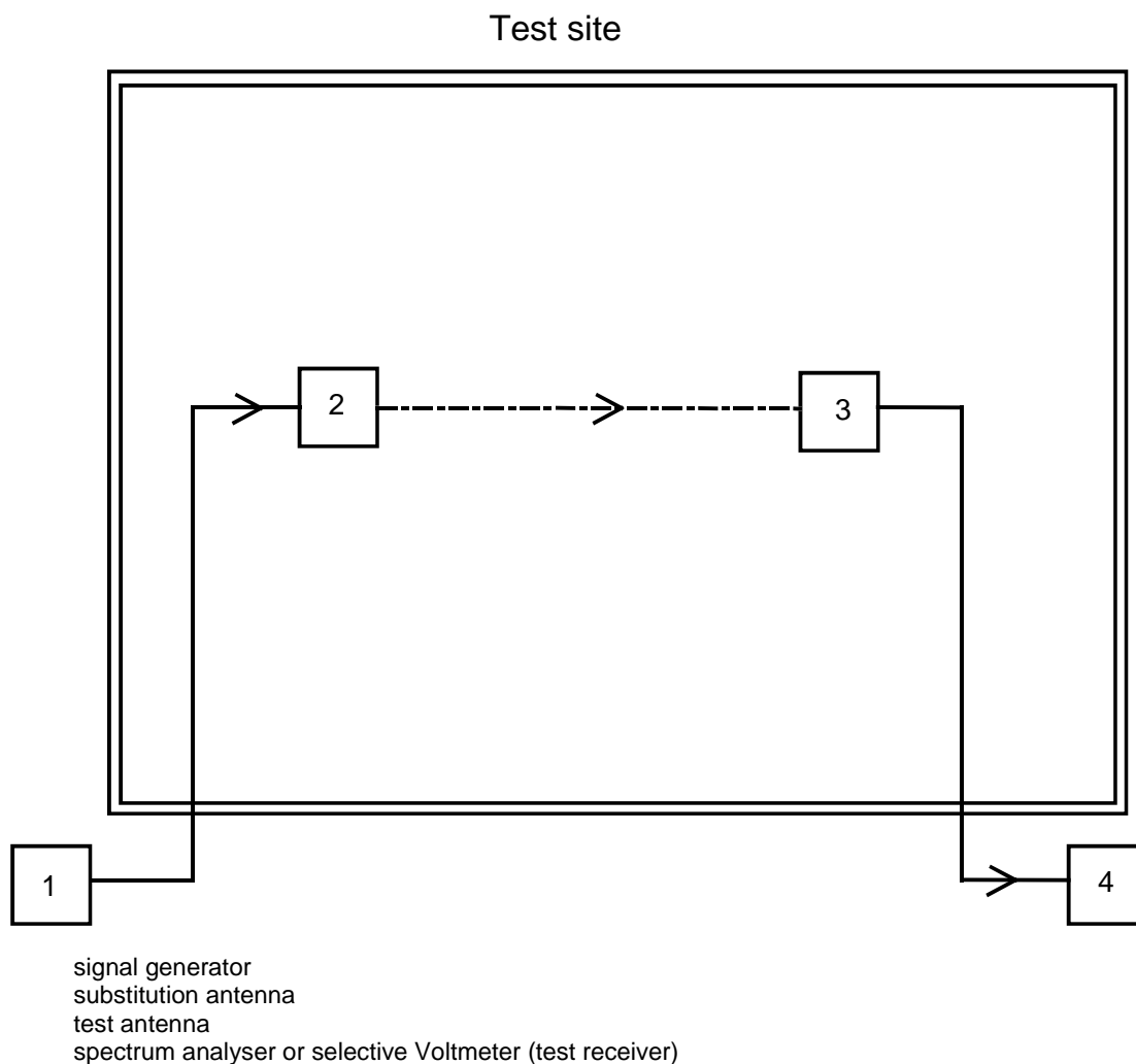
Figure 33: Measurement arrangement
