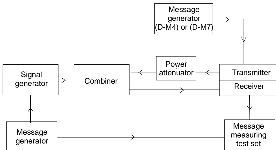
Figure 37: Measurement arrangement
