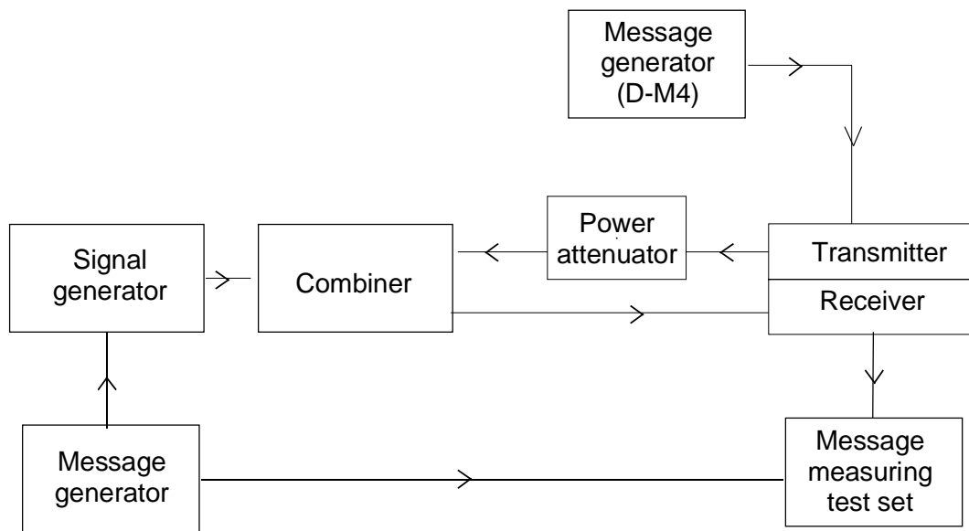
Figure 37: Measurement arrangement
