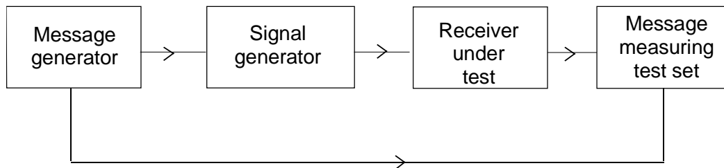
Figure 21: Measurement arrangement
