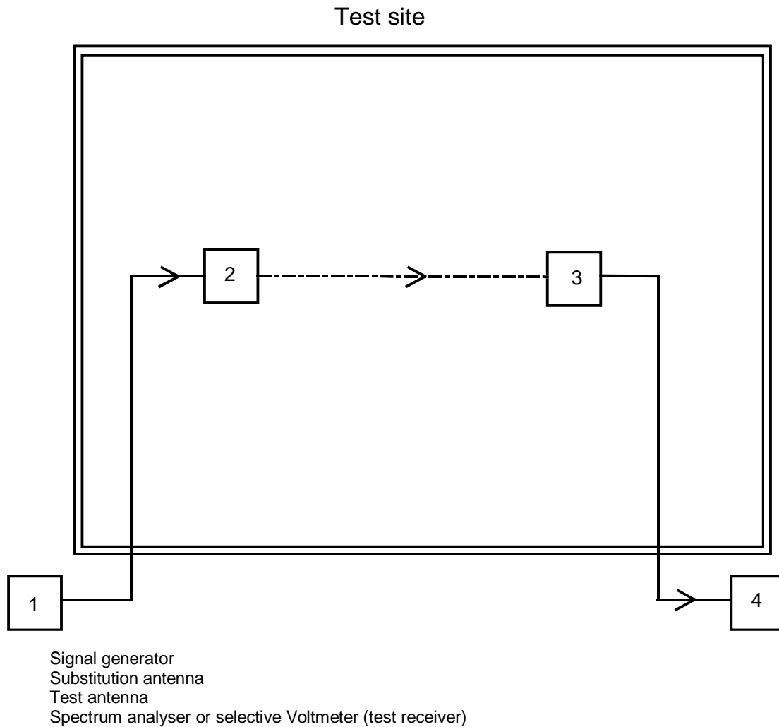
Figure 11: Measurement arrangement
