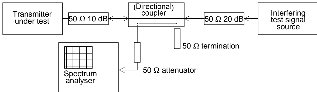
Figure 12: Measurement arrangement
