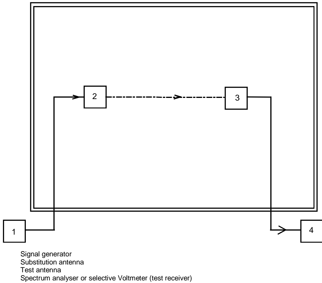
Figure 6: Measurement arrangement
