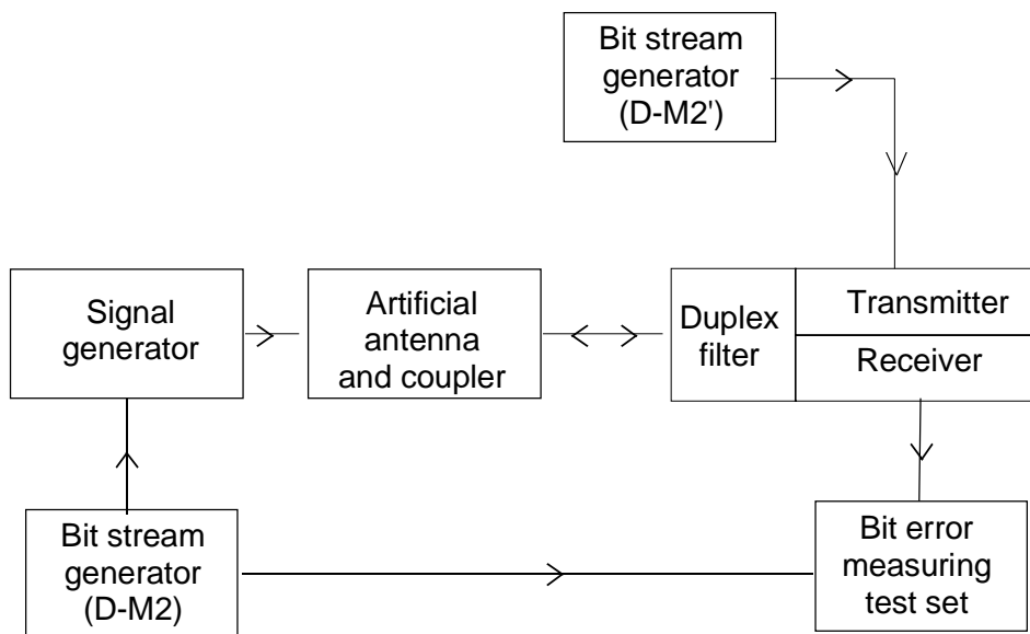
Figure 34: Measurement arrangement
