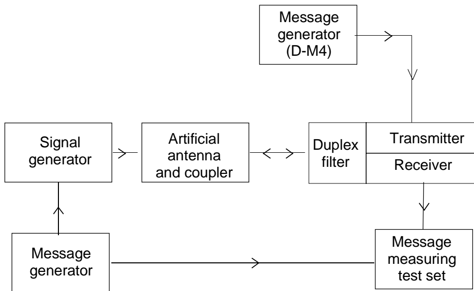
Figure 36: Measurement arrangement
