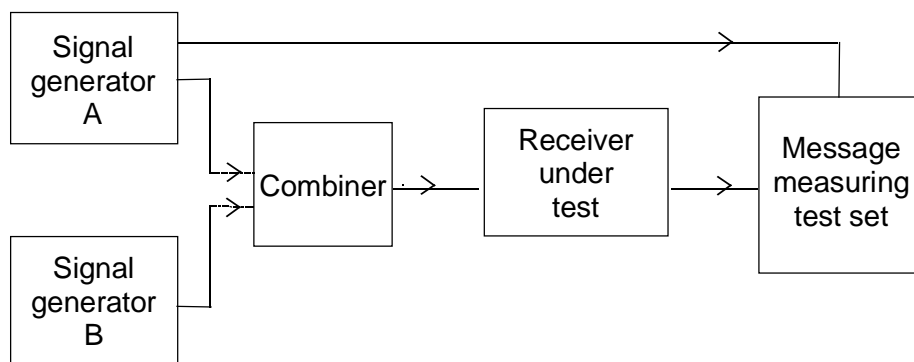
Figure 30: Measurement arrangement
