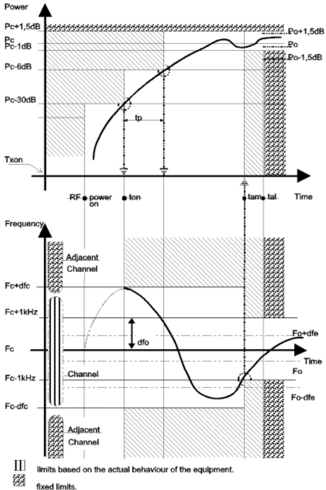
Figure 14: Transmitter attack time according to clause 8.8.1 b) and transient behaviour during switch-on (case where the attack time is given by the behaviour of the frequency)
