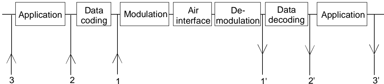
Figure 2: Test points for bit stream measurements
