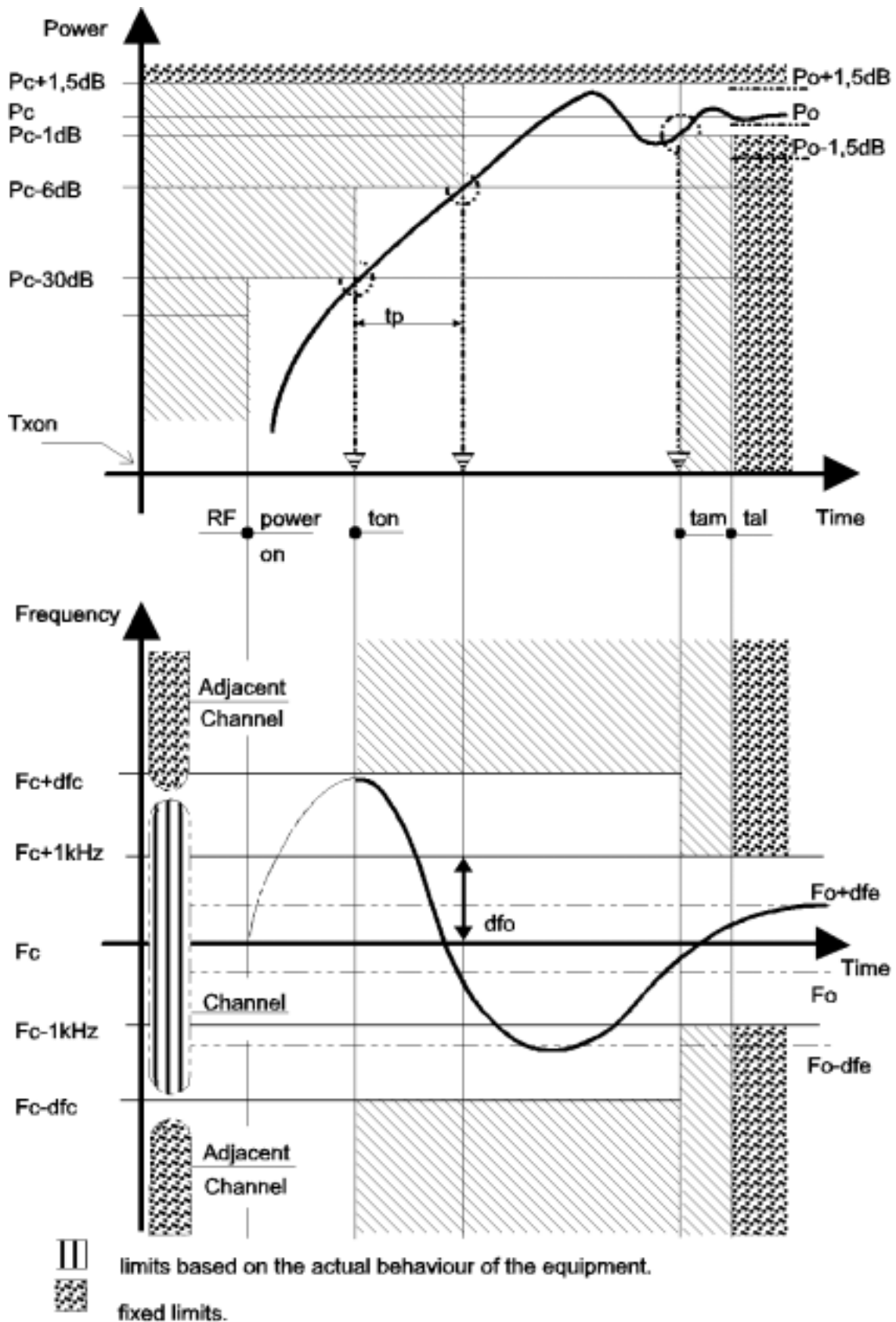
Figure 13: Transmitter attack time according to clause 8.8.1 a) and transient behaviour during switch-on (case where the attack time is given by the behaviour of the power rise)
