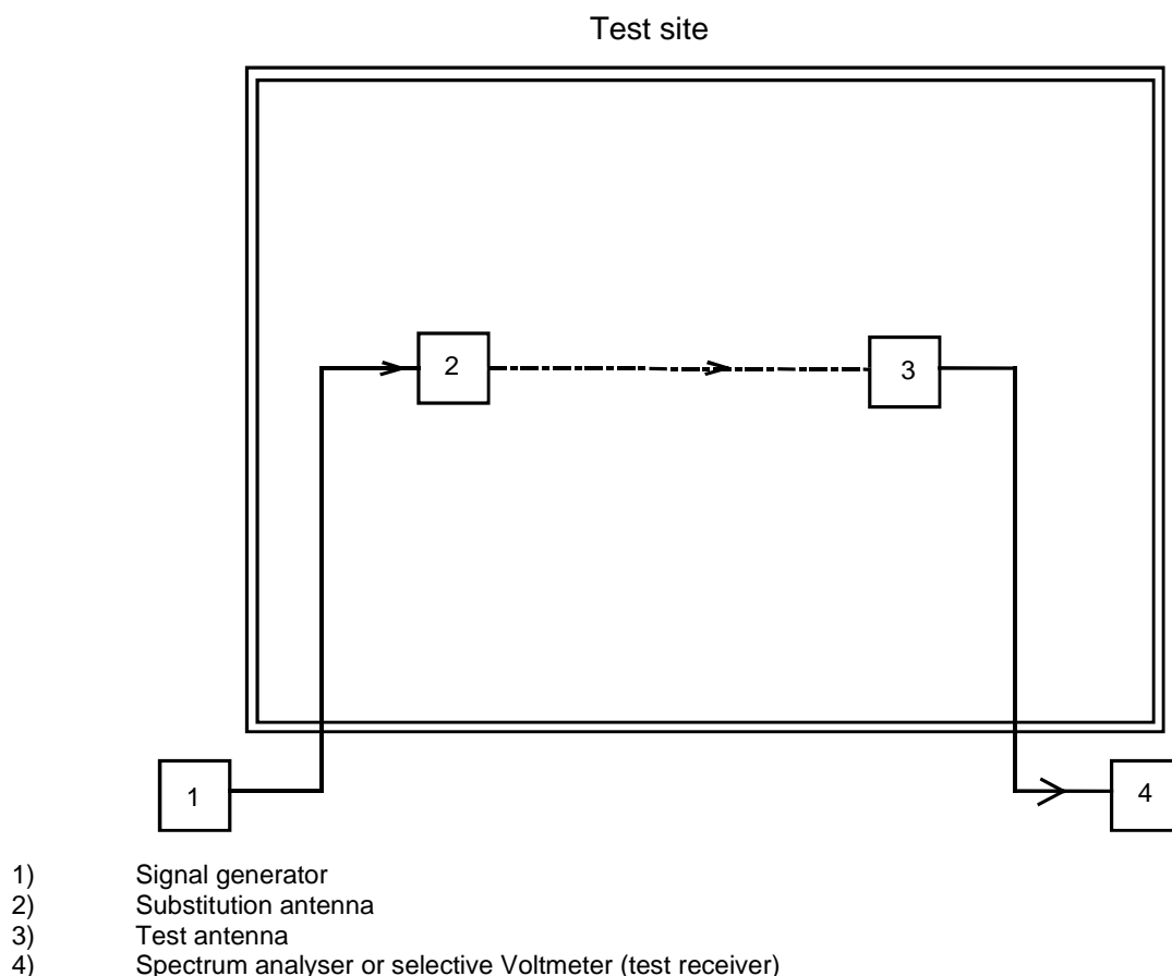
Figure 6: Measurement arrangement
