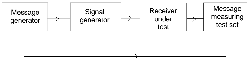
Figure 20: Measurement arrangement
