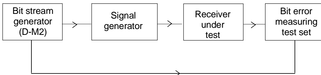
Figure 17: Measurement arrangement
