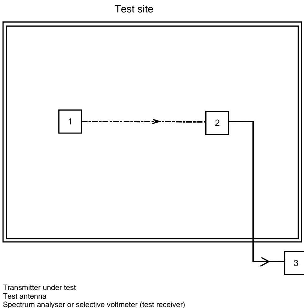
Figure 9: Measurement arrangement
