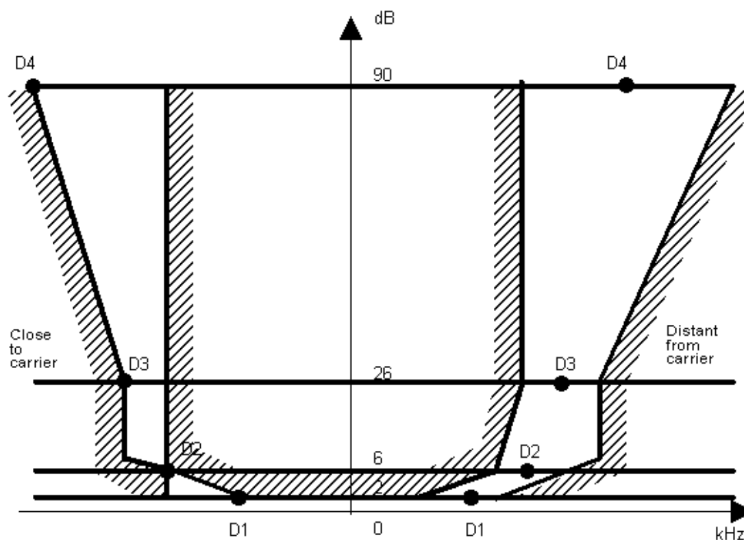
Figure C.1: IF filter
