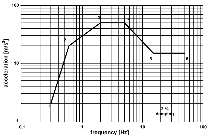
Figure 7: Earthquake Response Spectrum
