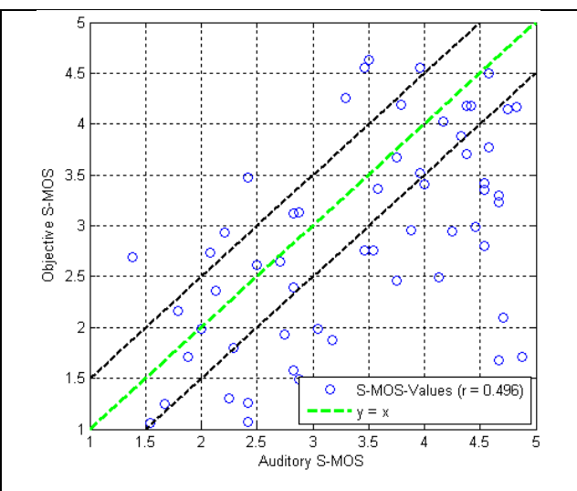
Figure J.12: Objective vs. Auditory S-MOS for Czech samples calculated with regression coefficients optimized for French data
