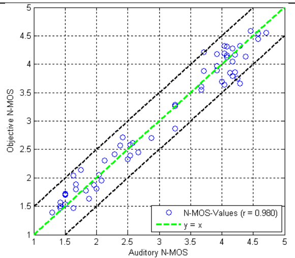
Figure J.10: Objective vs. Auditory N-MOS for Czech samples calculated with regression coefficients optimized for Czech data
