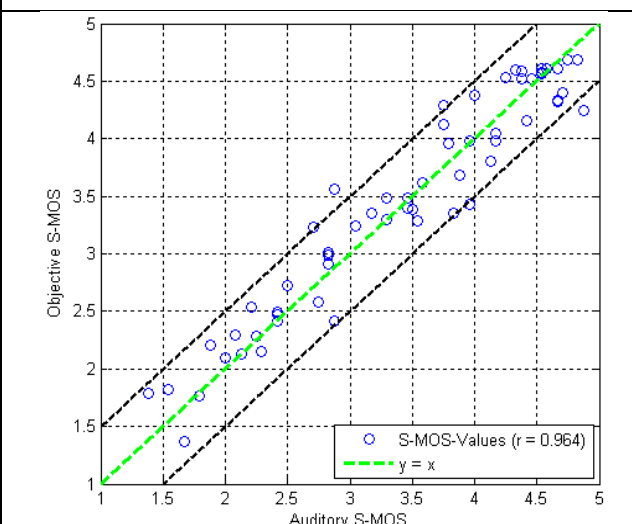
Figure J.14: Objective vs. Auditory S-MOS for Czech samples calculated with regression coefficients optimized for Czech data
