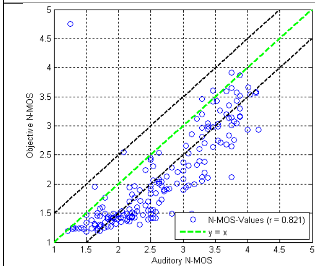
Figure J.9: Objective vs. Auditory N-MOS for French samples calculated with regression coefficients optimized for Czech data
