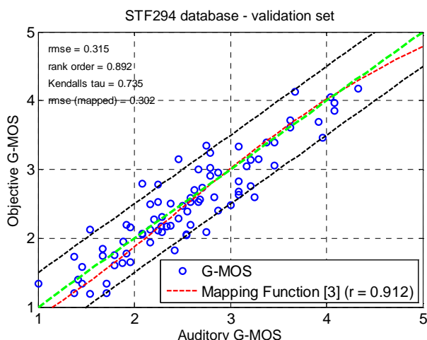
Figure 7.5: Left: Objectively calculated G-MOS versus auditory G-MOS for validation conditions
