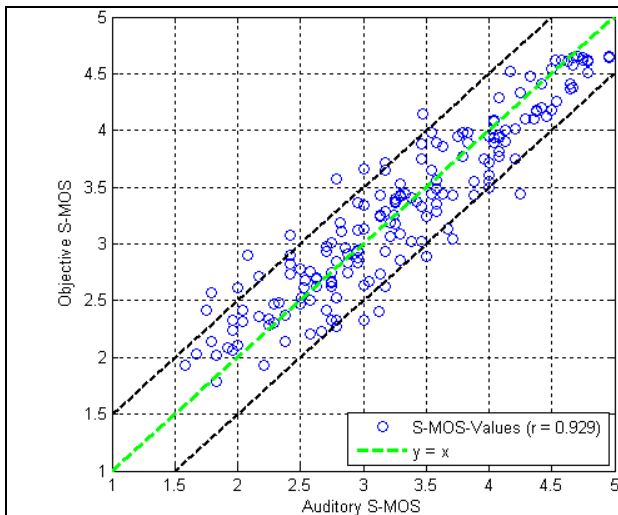
Figure J.11: Objective vs. Auditory S-MOS for French samples calculated with regression coefficients optimized for French data
