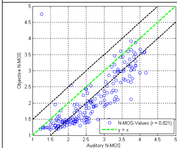
Figure J.9: Objective vs. Auditory N-MOS for French samples calculated with regression coefficients optimized for Czech data
