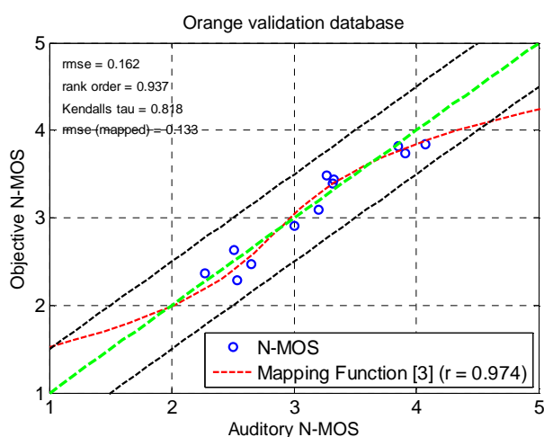
Figure 7.7: Left: Objectively calculated N-MOS versus auditory N-MOS for validation conditions
