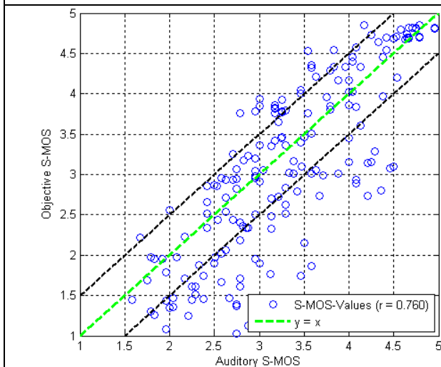
Figure J.13: Objective vs. Auditory S-MOS for French samples calculated with regression coefficients optimized for Czech data
