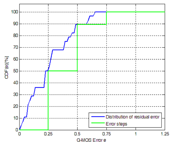
Figure J.24: Objectively CDF of residual error versus G-MOS error e for Czech validation conditions
