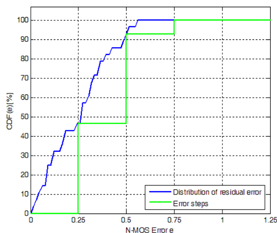
Figure J.20: Objectively CDF of residual error versus N-MOS error e for Czech validation conditions
