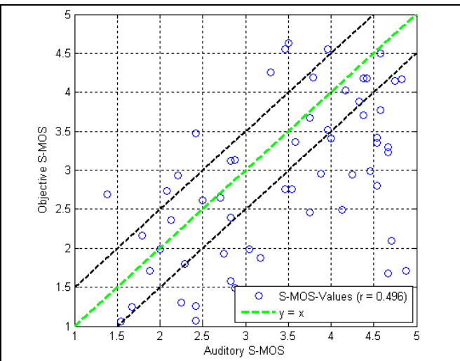
Figure J.12: Objective vs. Auditory S-MOS for Czech samples calculated with regression coefficients optimized for French data
