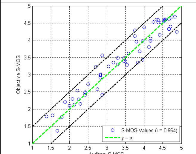
Figure J.14: Objective vs. Auditory S-MOS for Czech samples calculated with regression coefficients optimized for Czech data
