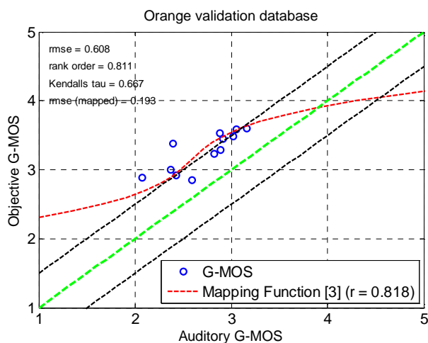
Figure 7.11: Left: Objectively calculated G-MOS versus auditory G-MOS for validation conditions
