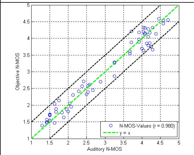
Figure J.10: Objective vs. Auditory N-MOS for Czech samples calculated with regression coefficients optimized for Czech data
