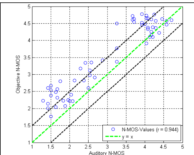
Figure J.8: Objective vs. Auditory N-MOS for Czech samples calculated with regression coefficients optimized for French data
