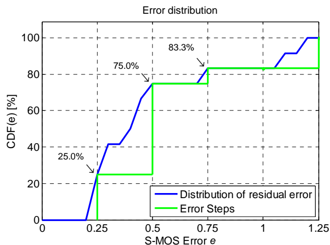
Figure 7.10: Objectively CDF of residual error versus S-MOS error e for validation conditions
