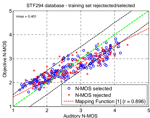
Figure C.1: Objective versus auditory N-MOS for all French training conditions
