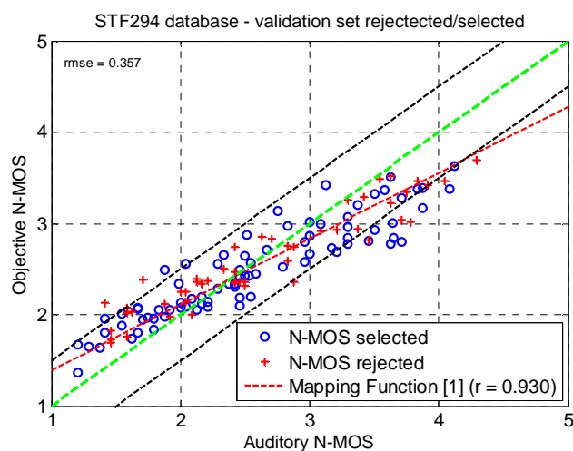
Figure C.2: Objective versus auditory N-MOS for all French validation conditions
