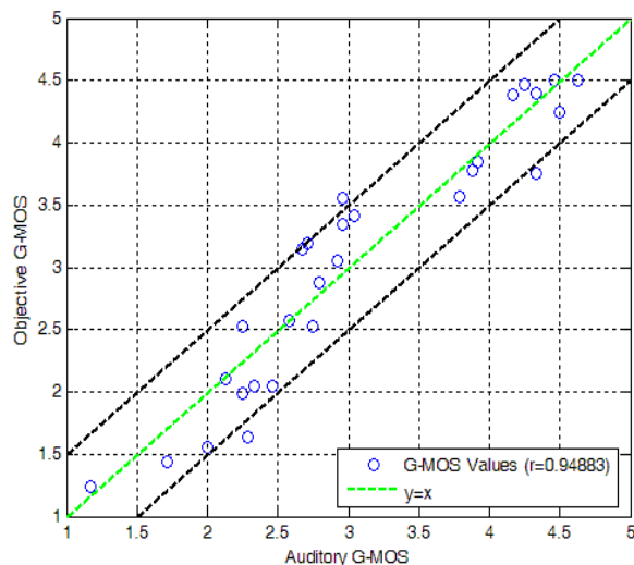
Figure J.23: Objectively calculated S-MOS versus auditory G-MOS for Czech validation conditions
