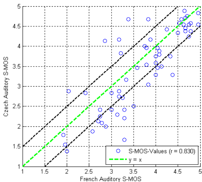
Figure J.2: Scatter plot of the French data vs. the Czech data, S-MOS, after experts' selection (only data selected for both languages)
