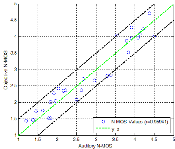
Figure J.19: Objectively calculated N-MOS versus auditory N-MOS for Czech validation conditions
