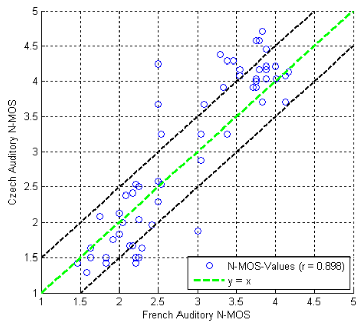
Figure J.4: Scatter plot of the French data vs. the Czech data, N-MOS, after experts' selection (only data selected for both languages)
