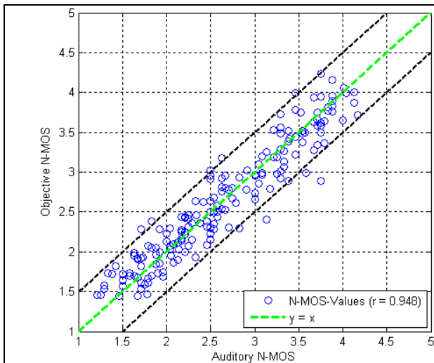
Figure J.7: Objective vs. Auditory N-MOS for French samples calculated with regression coefficients optimized for French data
