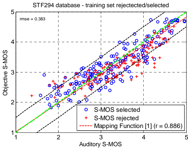
Figure C.3: Objective versus auditory S-MOS for all French training conditions
