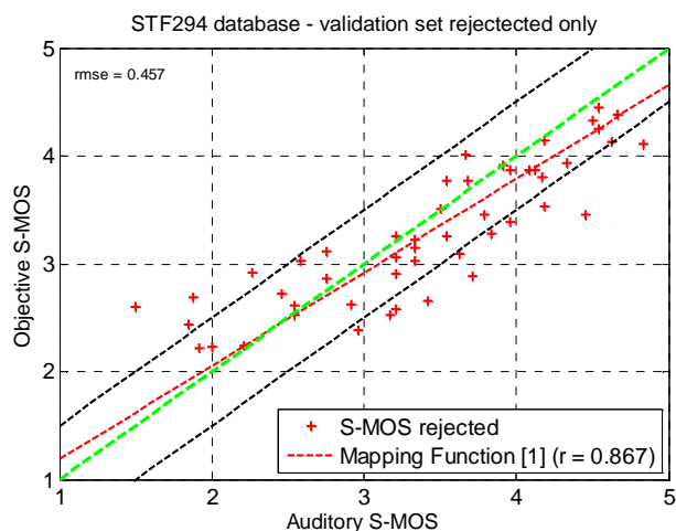
Figure D.4: Objective versus auditory S-MOS only for validation data not used for the model development
