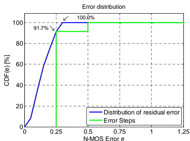
Figure 7.8: Objectively CDF of residual error versus N-MOS error e for validation conditions
