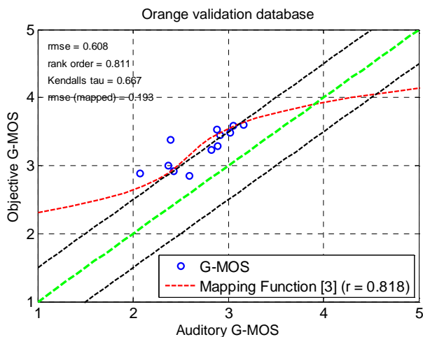
Figure 7.11: Left: Objectively calculated G-MOS versus auditory G-MOS for validation conditions
