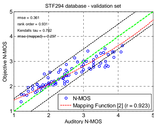
Figure 7.1: Left: Objectively calculated N-MOS versus auditory N-MOS for validation conditions
