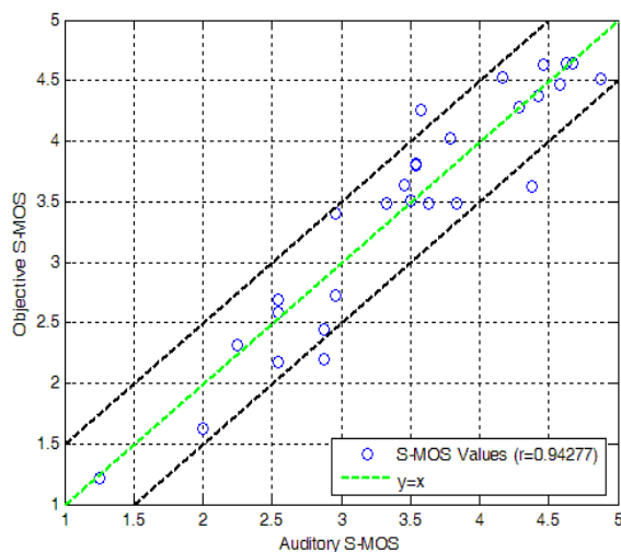
Figure J.21: Objectively calculated S-MOS versus auditory S-MOS for Czech validation conditions
