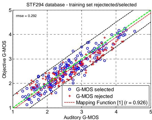
Figure C.5: Objective versus auditory G-MOS for all French training conditions
