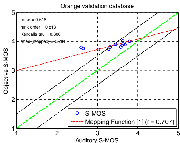
Figure 7.9: Left: Objectively calculated S-MOS versus auditory S-MOS for validation conditions
