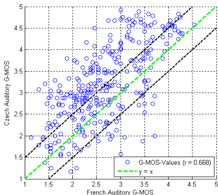
Figure J.5: Scatter plot of the French data vs. the Czech data for the different conditions, G-MOS, before experts' selection
