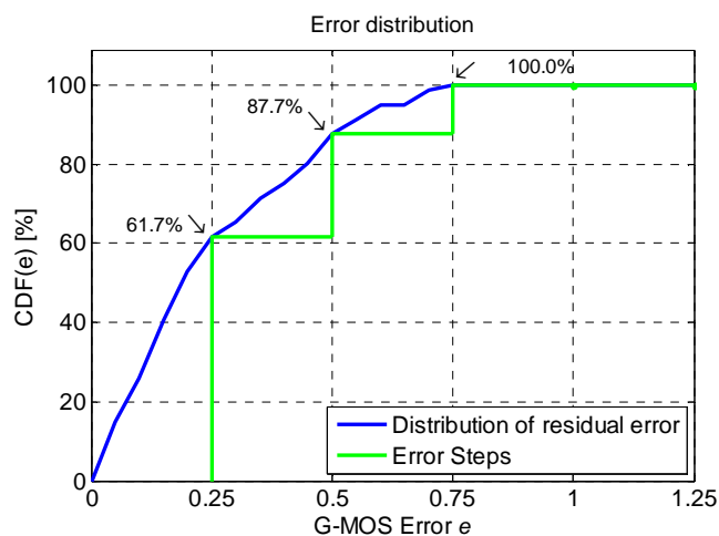
Figure 7.6: Objectively CDF of residual error versus G-MOS error e for validation conditions
