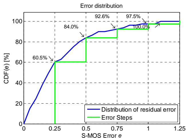
Figure 7.4: Objectively CDF of residual error versus S-MOS error e for validation conditions
