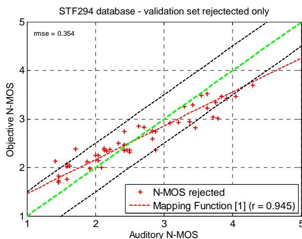
Figure D.2: Objective versus auditory N-MOS only for validation data not used for the model development
