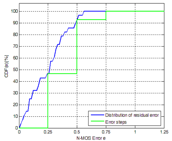
Figure J.20: Objectively CDF of residual error versus N-MOS error e for Czech validation conditions
