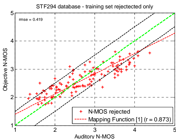
Figure D.1: Objective versus auditory N-MOS only for training data not used for the model development
