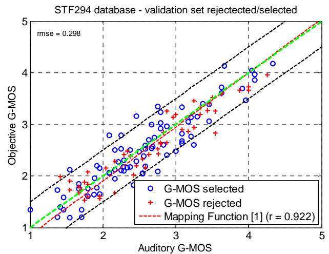
Figure C.6: Objective versus auditory G-MOS for all French validation conditions
