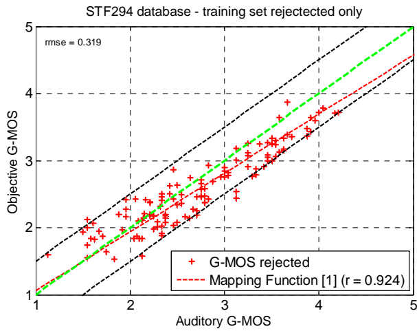
Figure D.5: Objective versus auditory G-MOS only for training data not used for the model development
