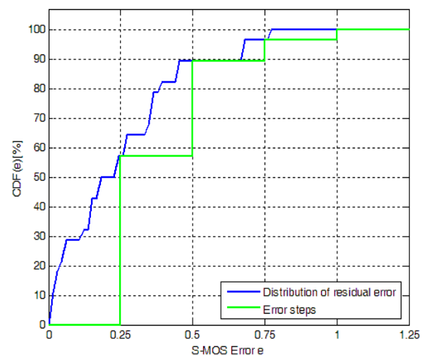
Figure J.22: Objectively CDF of residual error versus S-MOS error e for Czech validation conditions
