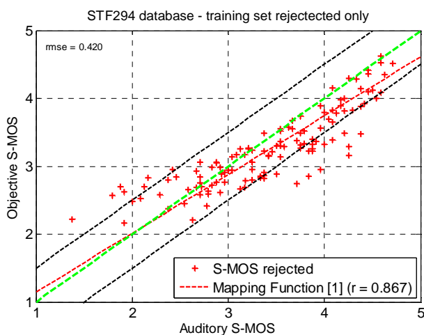
Figure D.3: Objective versus auditory S-MOS only for training data not used for the model development
