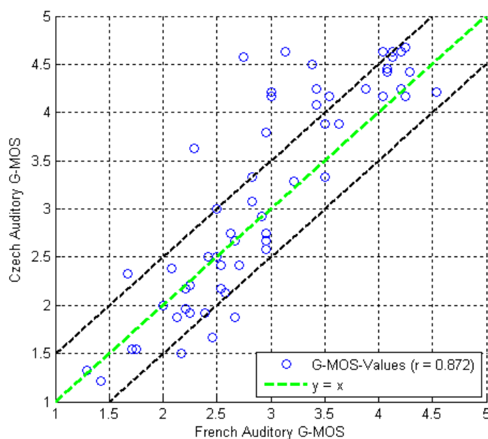
Figure J.6: Scatter plot of the French data vs. the Czech data, G-MOS, after experts' selection (only data selected for both languages)
