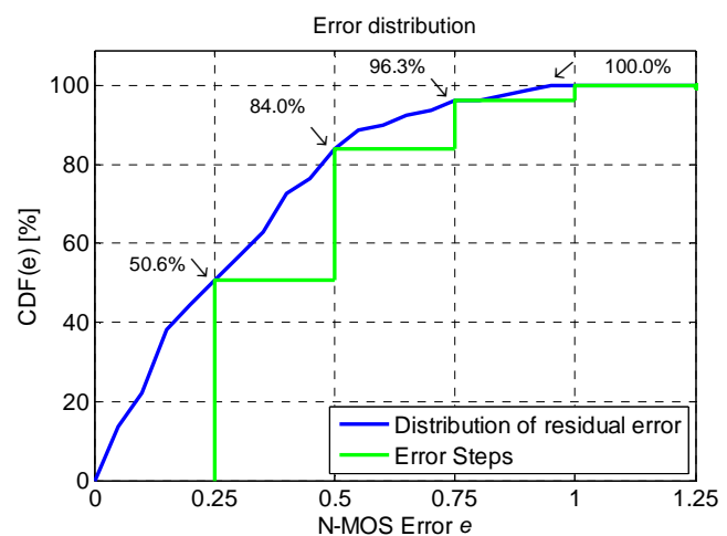
Figure 7.2: Objectively CDF of residual error versus N-MOS error e for validation conditions
