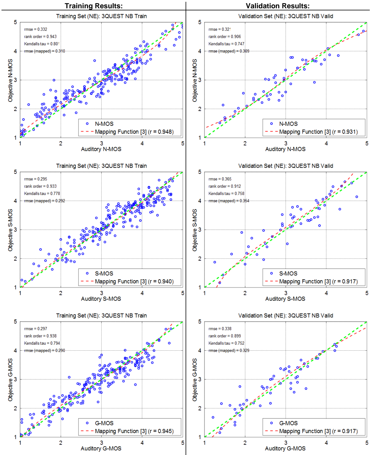
Figure 8.2: HEAD acoustics NB Database - Comparison subjective vs. Objective data
