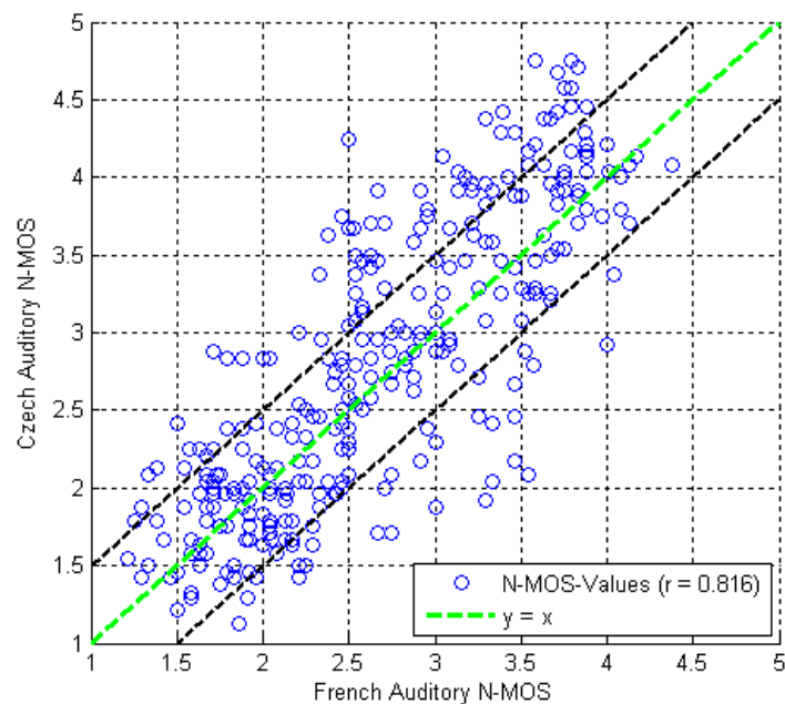
Figure J.3: Scatter plot of the French data vs. the Czech data for the different conditions, N-MOS, before experts' selection
