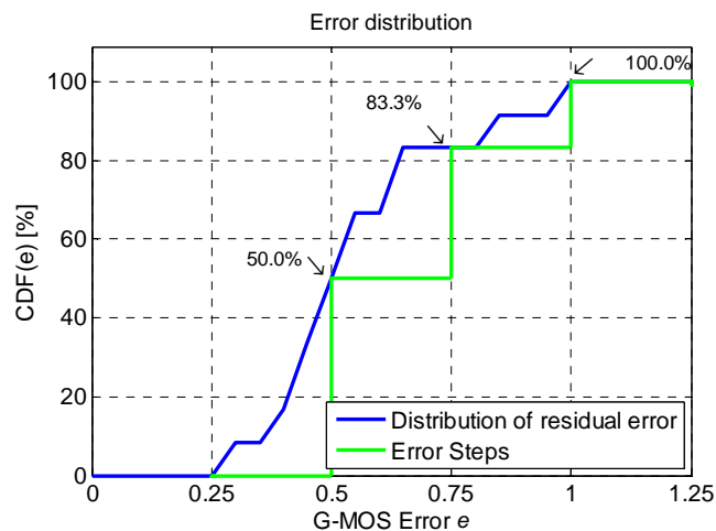
Figure 7.12: Objectively CDF of residual error versus G-MOS error e for validation conditions
