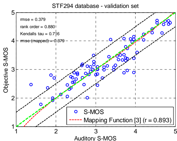
Figure 7.3: Left: Objectively calculated S-MOS versus auditory S-MOS for validation conditions
