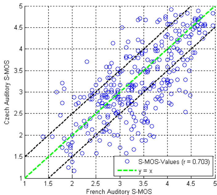
Figure J.1: Scatter plot of the French data vs. the Czech data for the different conditions, S-MOS, before experts' selection
