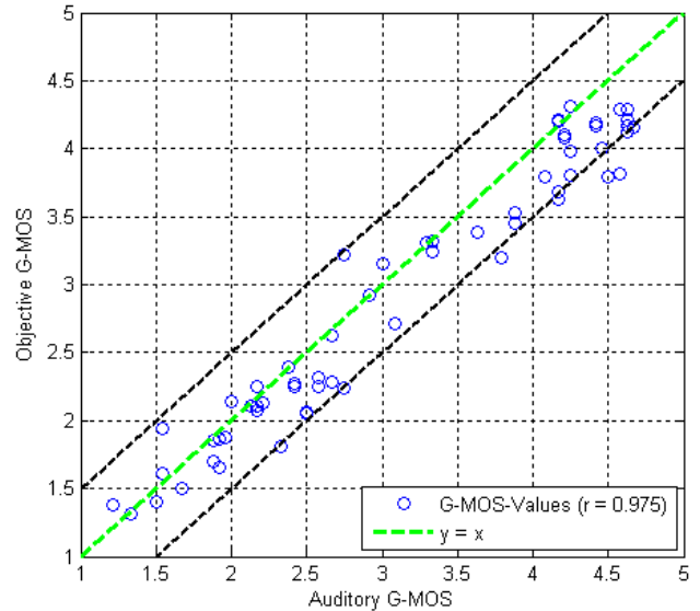
Figure J.26: Objective vs. Auditory G-MOS for Czech samples calculated with regression coefficients optimized for French data (N-MOS and S-MOS optimized for Czech data)
