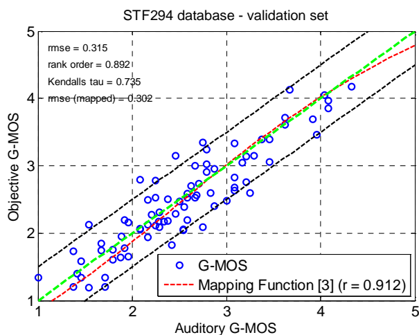
Figure 7.5: Left: Objectively calculated G-MOS versus auditory G-MOS for validation conditions
