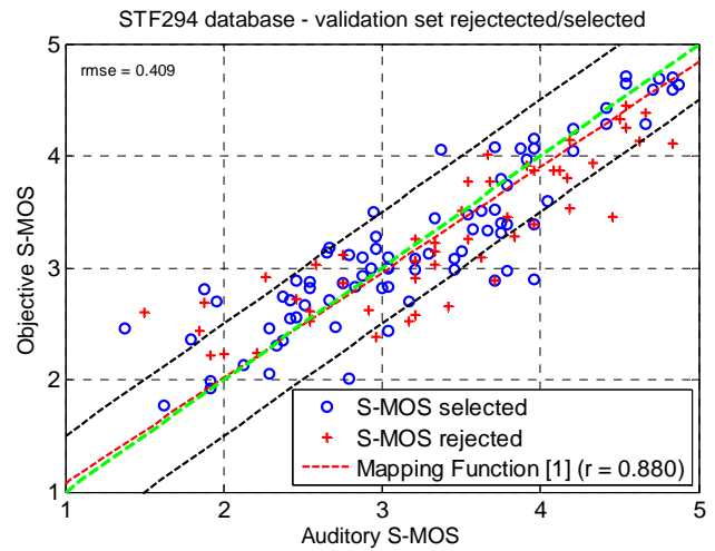
Figure C.4: Objective versus auditory S-MOS for all French validation conditions
