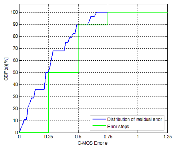
Figure J.24: Objectively CDF of residual error versus G-MOS error e for Czech validation conditions
