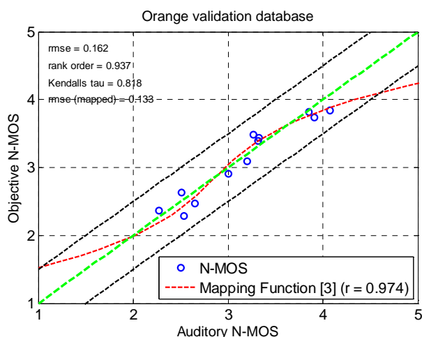
Figure 7.7: Left: Objectively calculated N-MOS versus auditory N-MOS for validation conditions
