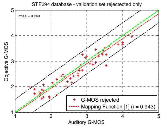
Figure D.6: Objective versus auditory G-MOS only for validation data not used for the model development
