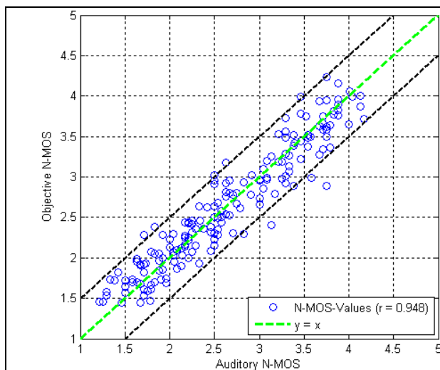
Figure 6.13: Objective vs. auditory N-MOS for French samples calculated with regression coefficients optimized for French data
