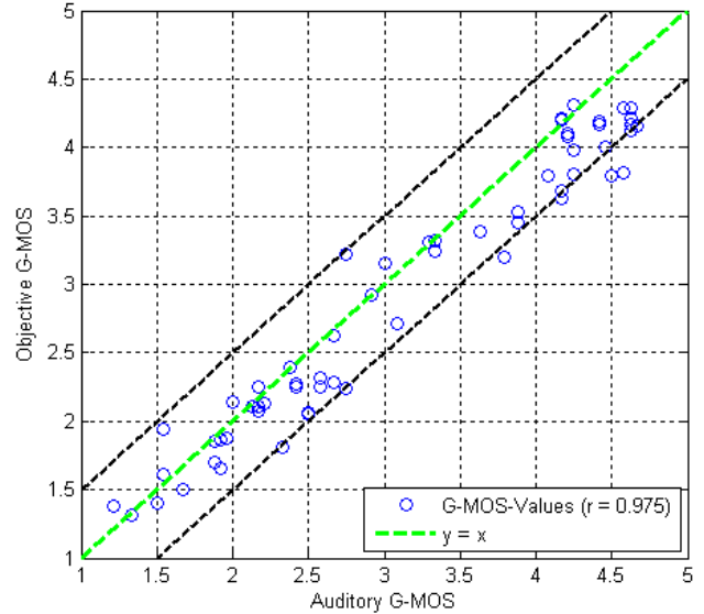
Figure 6.26: Objective vs. auditory G-MOS for Czech samples calculated with regression coefficients optimized for French data (N-MOS and S-MOS optimized for Czech data)
