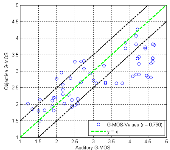
Figure 6.22: Objective vs. auditory G-MOS for Czech samples calculated with regression coefficients optimized for French data (N-MOS and S-MOS optimized for French data)
