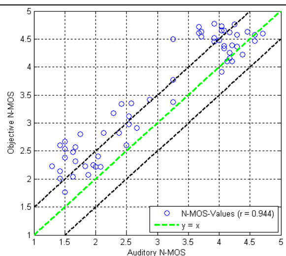
Figure 6.14: Objective vs. auditory N-MOS for Czech samples calculated with regression coefficients optimized for French data
