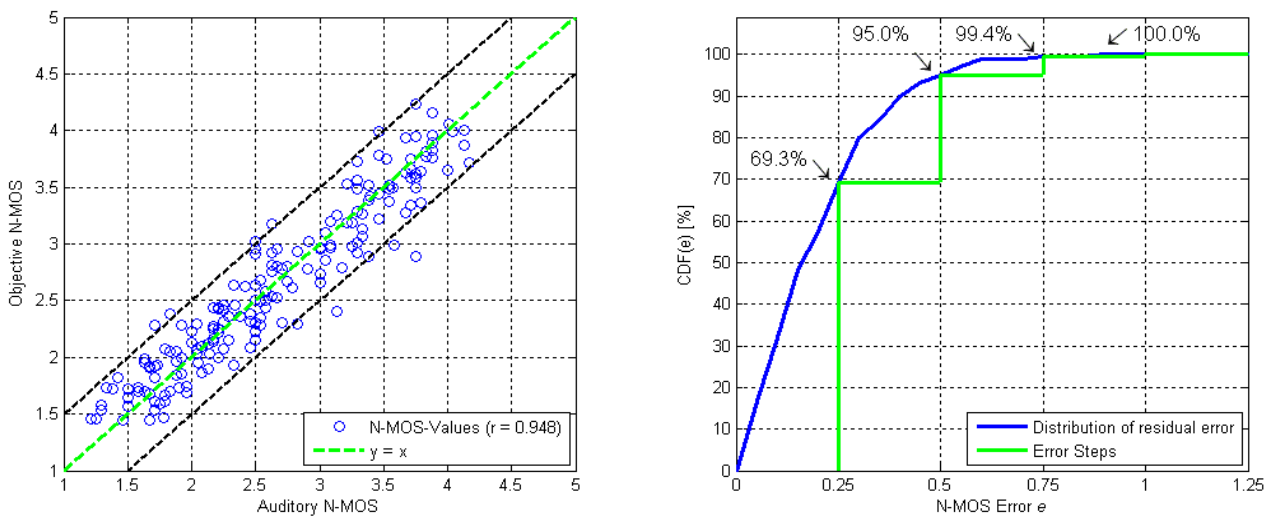
Figure 6.8: Left: Objectively calculated N-MOS versus auditory N-MOS; Right: CDF of residual error versus N-MOS error e
