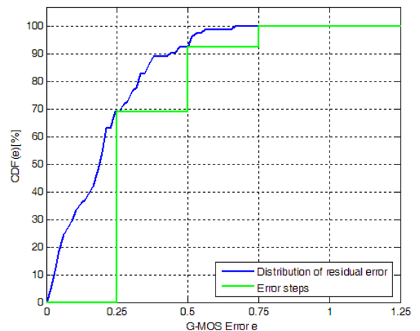
Figure 7.12: Objectively CDF of residual error versus G-MOS error e for French validation conditions
