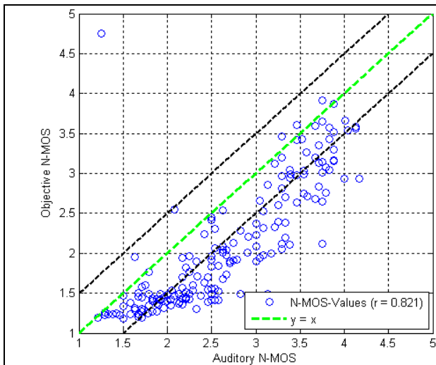
Figure 6.15: Objective vs. auditory N-MOS for French samples calculated with regression coefficients optimized for Czech data
