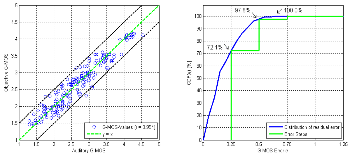
Figure 6.12: Left: Objectively calculated G-MOS versus auditory G-MOS; Right: CDF of residual error versus G-MOS error e
