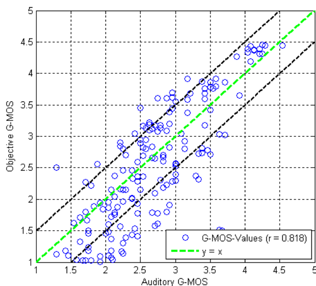
Figure 6.23: Objective vs. auditory G-MOS for French samples calculated with regression coefficients optimized for Czech data (N-MOS and S-MOS optimized for Czech data)
