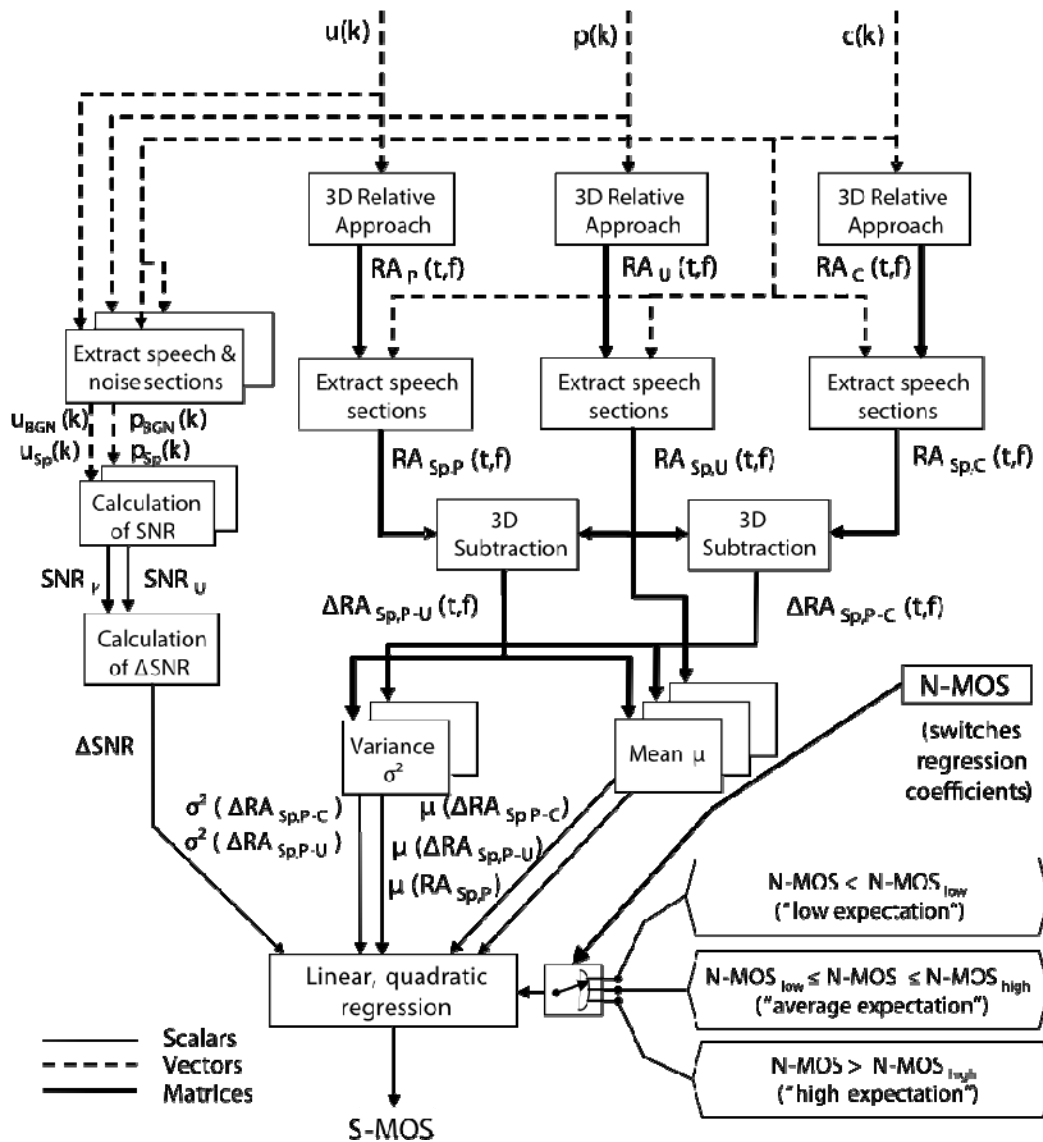
Figure 6.9: Block diagram of S-MOS calculation algorithm; u(k) unprocessed signal, p(k) processed signal, c(k) clean speech signal
