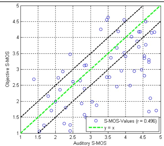
Figure 6.18: Objective vs. auditory S-MOS for Czech samples calculated with regression coefficients optimized for French data
