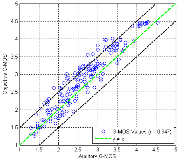
Figure 6.25: Objective vs. auditory G-MOS for French samples calculated with regression coefficients optimized for Czech data (N-MOS and S-MOS optimized for French data)
