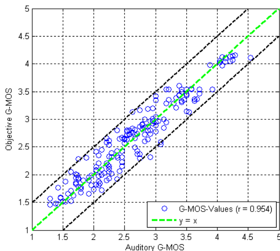
Figure 6.21: Objective vs. auditory G-MOS for French samples calculated with regression coefficients optimized for French data
