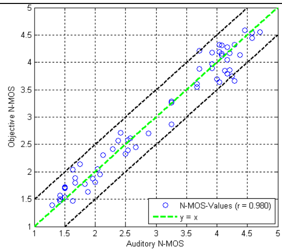
Figure 6.16: Objective vs. auditory N-MOS for Czech samples calculated with regression coefficients optimized for Czech data
