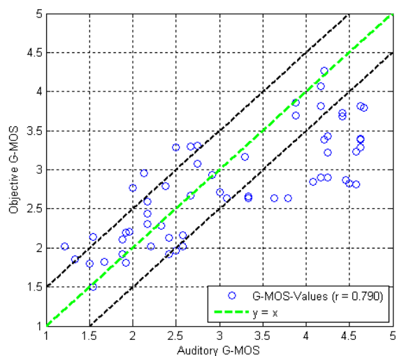
Figure 6.22: Objective vs. auditory G-MOS for Czech samples calculated with regression coefficients optimized for French data (N-MOS and S-MOS optimized for French data)
