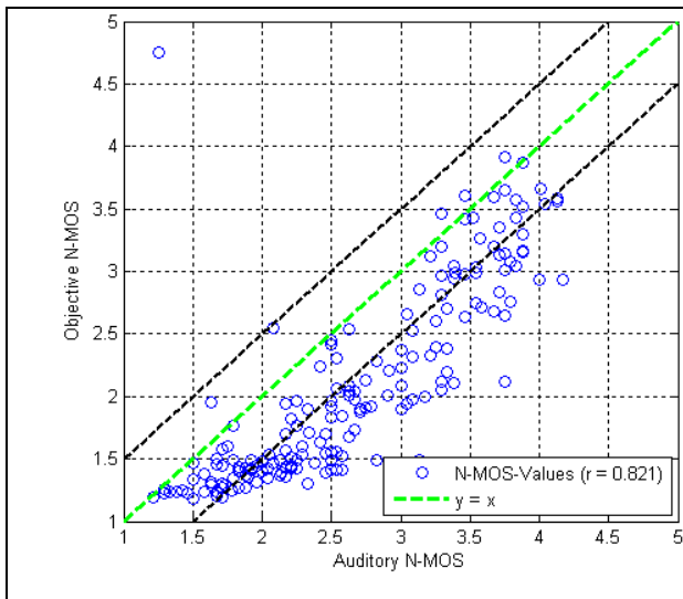
Figure 6.15: Objective vs. auditory N-MOS for French samples calculated with regression coefficients optimized for Czech data
