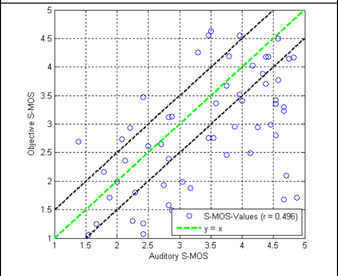
Figure 6.18: Objective vs. auditory S-MOS for Czech samples calculated with regression coefficients optimized for French data
