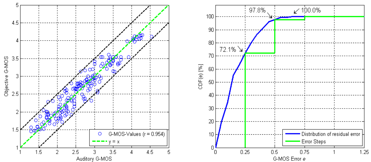
Figure 6.12: Left: Objectively calculated G-MOS versus auditory G-MOS; Right: CDF of residual error versus G-MOS error e
