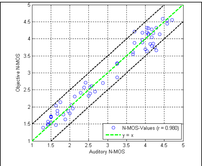
Figure 6.16: Objective vs. auditory N-MOS for Czech samples calculated with regression coefficients optimized for Czech data
