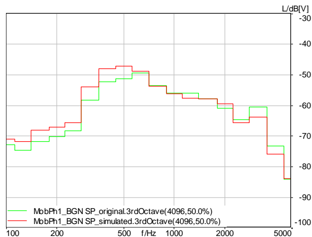
Figure 15: Power density spectra measured with a common mobile phone (with background noise signal processing) positioned at the artificial heads right ear
