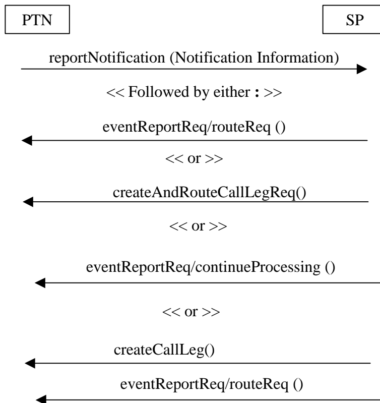
Figure 32: Reception of the originally dialled digits
