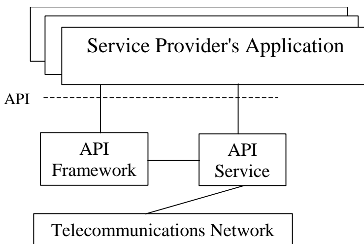
Figure 1: API Architecture
