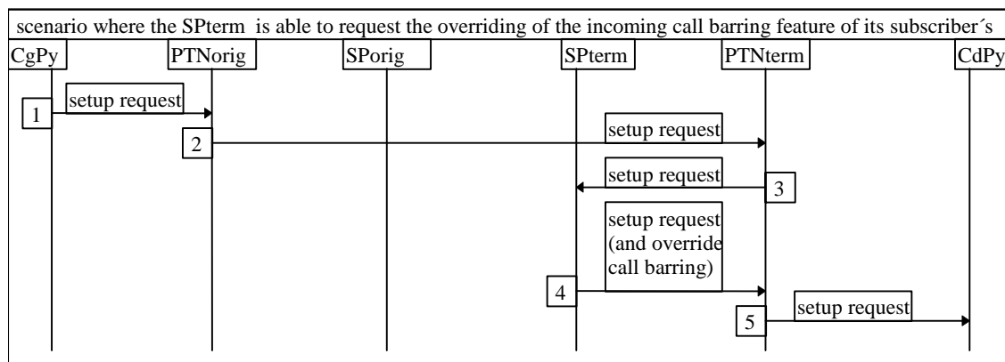
Figure 19: Overriding of the "incoming call barring" supplementary service
