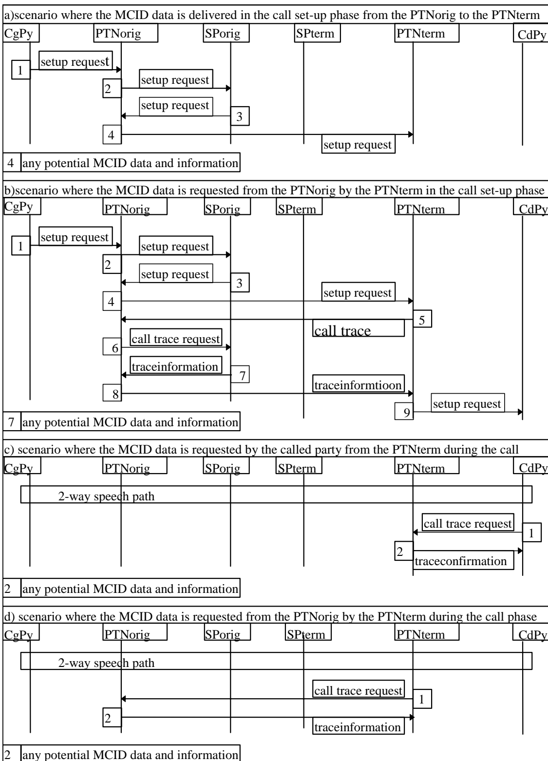
Figure 6: Relaying of the malicious call identification data of a received call
