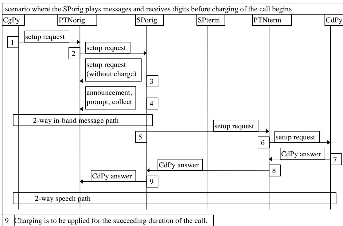
Figure 13: User interaction without service charging
