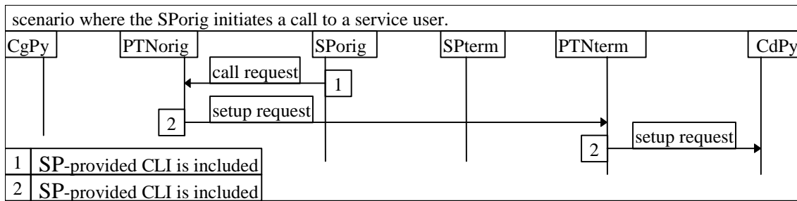
Figure 29: Provision of CLI information to an SP-initiated call
