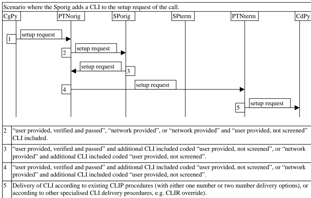
Figure 4: Addition of a calling line identity
