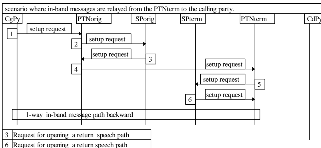
Figure 7: Return speech path connection from the PTNterm to the calling party
