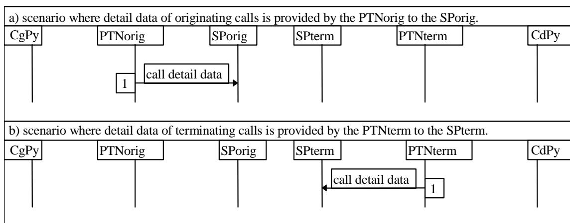
Figure 23: Event traceability
