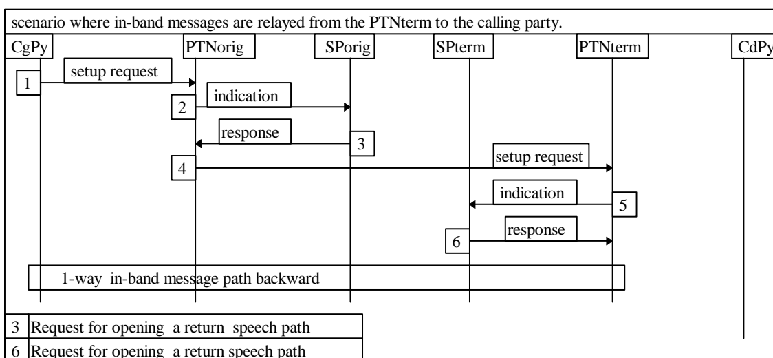
Figure 30: Return speech path connection from the PTNterm to the calling party
