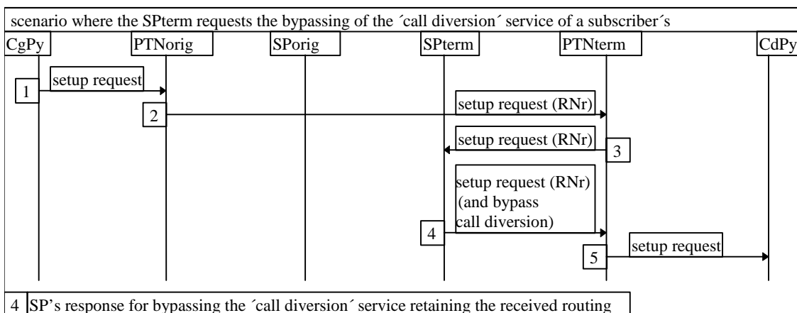
Figure 20: Bypassing of the call diversion supplementary service
