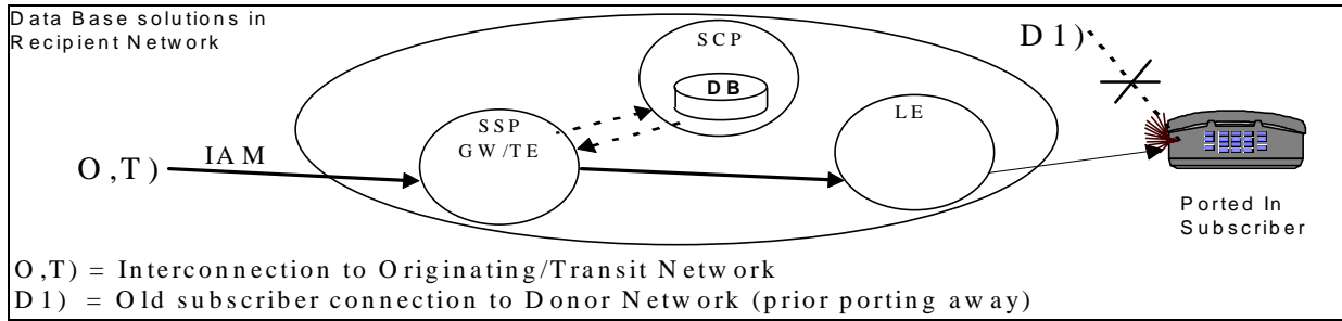
Figure 20: NP data stored switch external and queried by Recipient GW/TE Exchange(-s)
