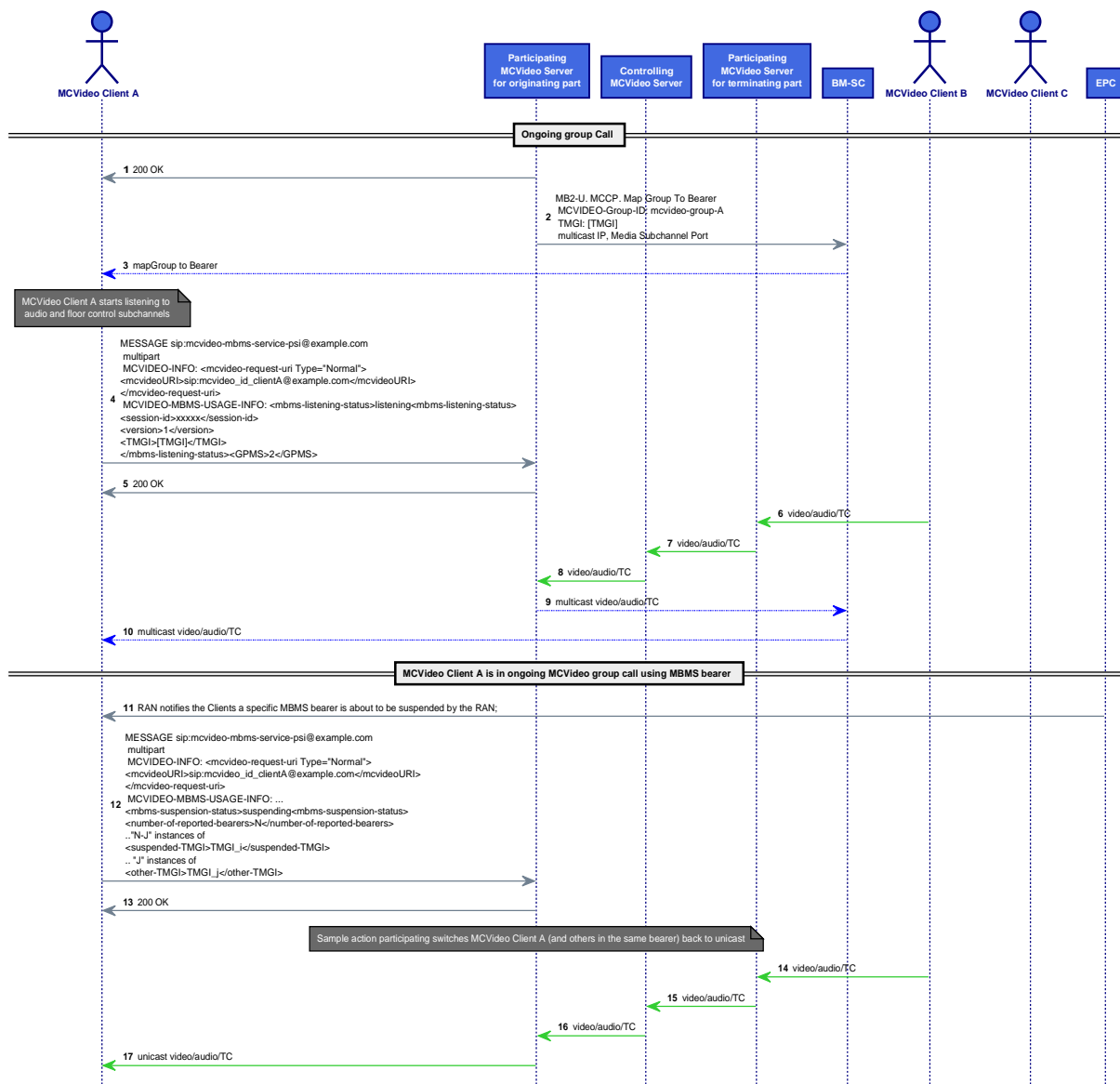
Figure 83l: EMBMS-MCVIDEO/SUSPENSION/01 Message Sequence
