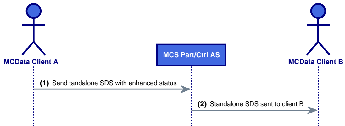
Figure 130: OS7.2 Message Sequence
