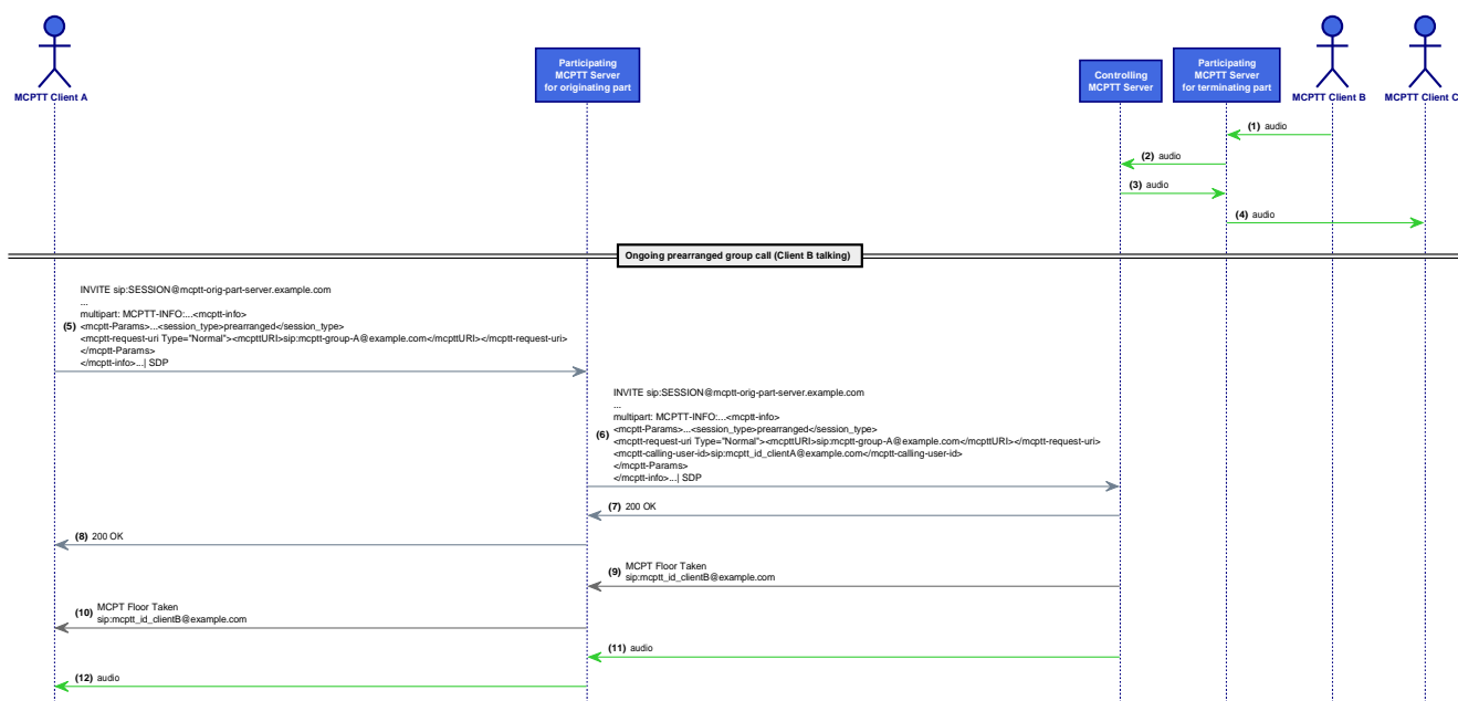
Figure 62c: CONN-MCPTT/ONN/GROUP/PREA/ONDEM/NFC/07 Message Sequence
