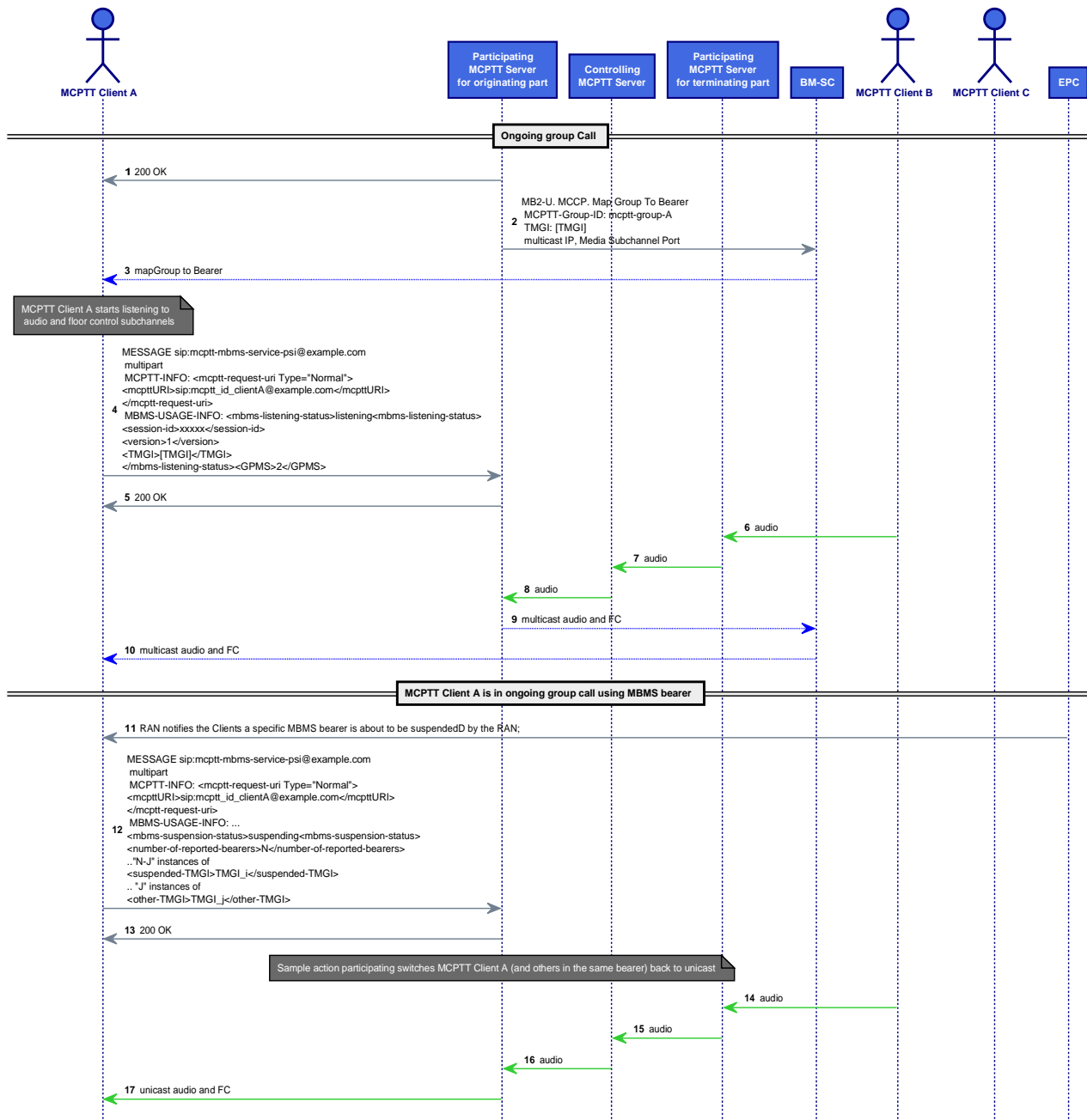
Figure 82b: EMBMS/SUSPENSION/01 Message Sequence
