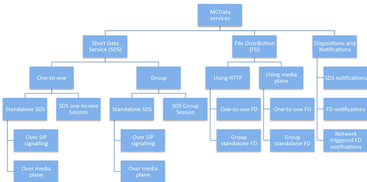
Figure 4: MCDATA services in Release 14 of ETSI TS 124 282 [8]
