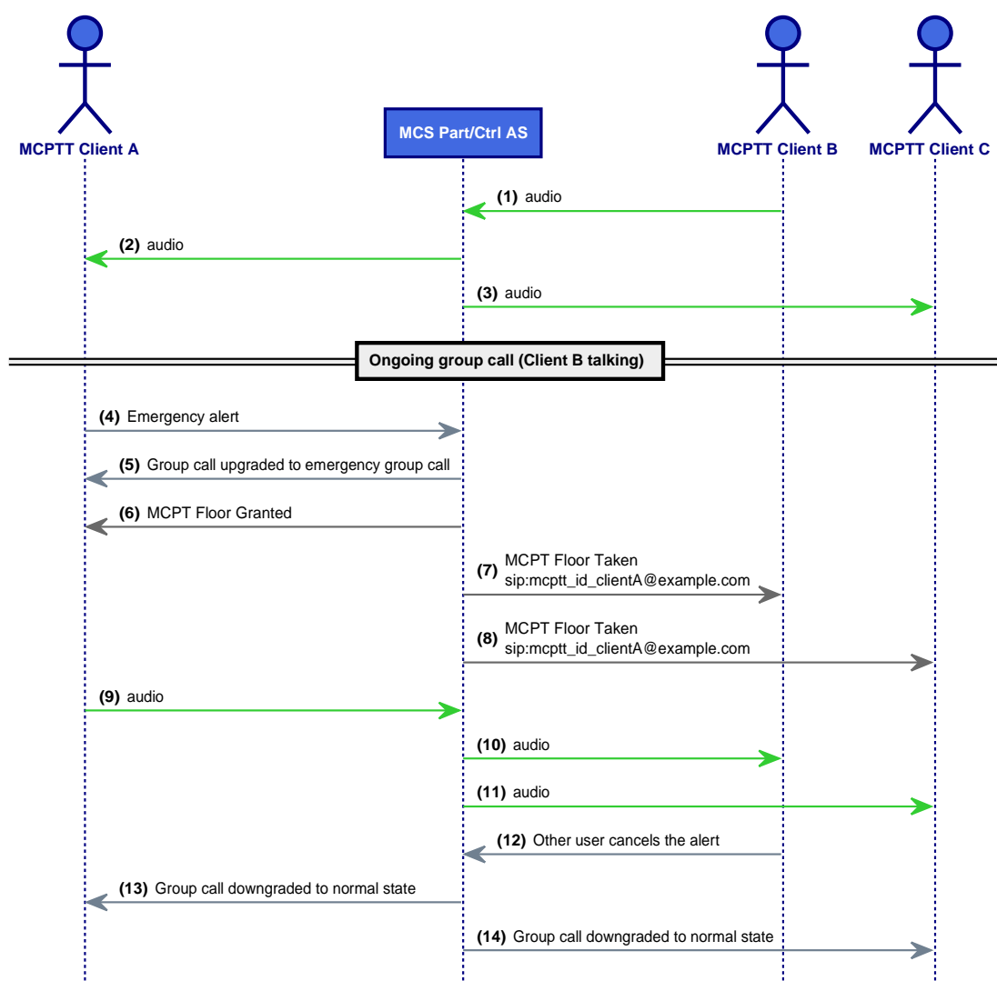
Figure 124: OS2 Message Sequence
