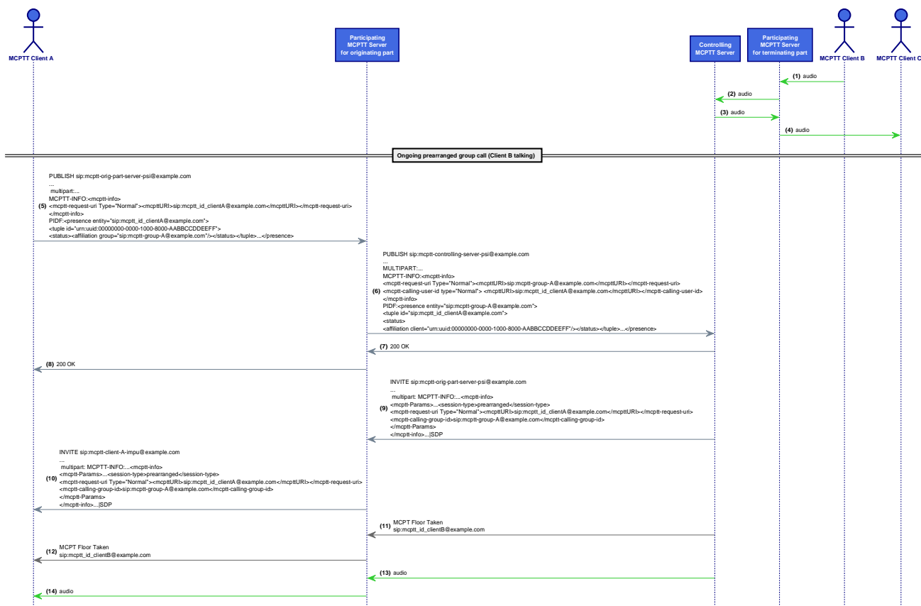
Figure 62a: CONN-MCPTT/ONN/GROUP/PREA/ONDEM/NFC/07 Message Sequence
