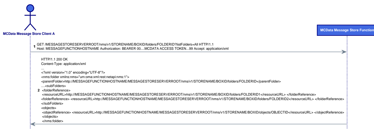
Figure 122mu: MCDATAMS/LIST/01 Message Sequence
