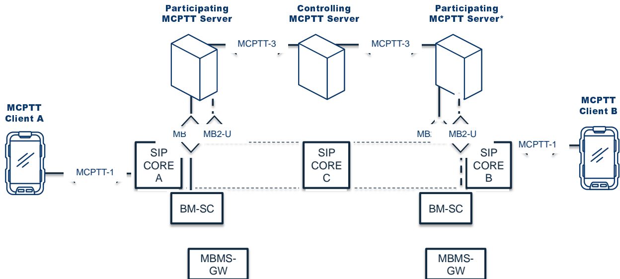
Figure 12: CFG_ONN_MULTI-MC-LTE-1 Application plane interfaces
