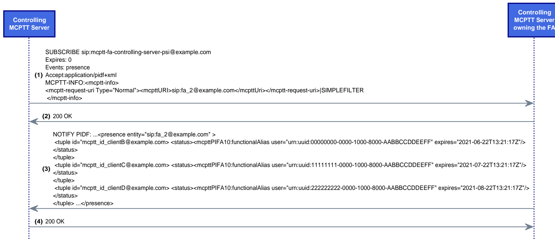
Figure 122fa: FA/RESOL/01Message Sequence
