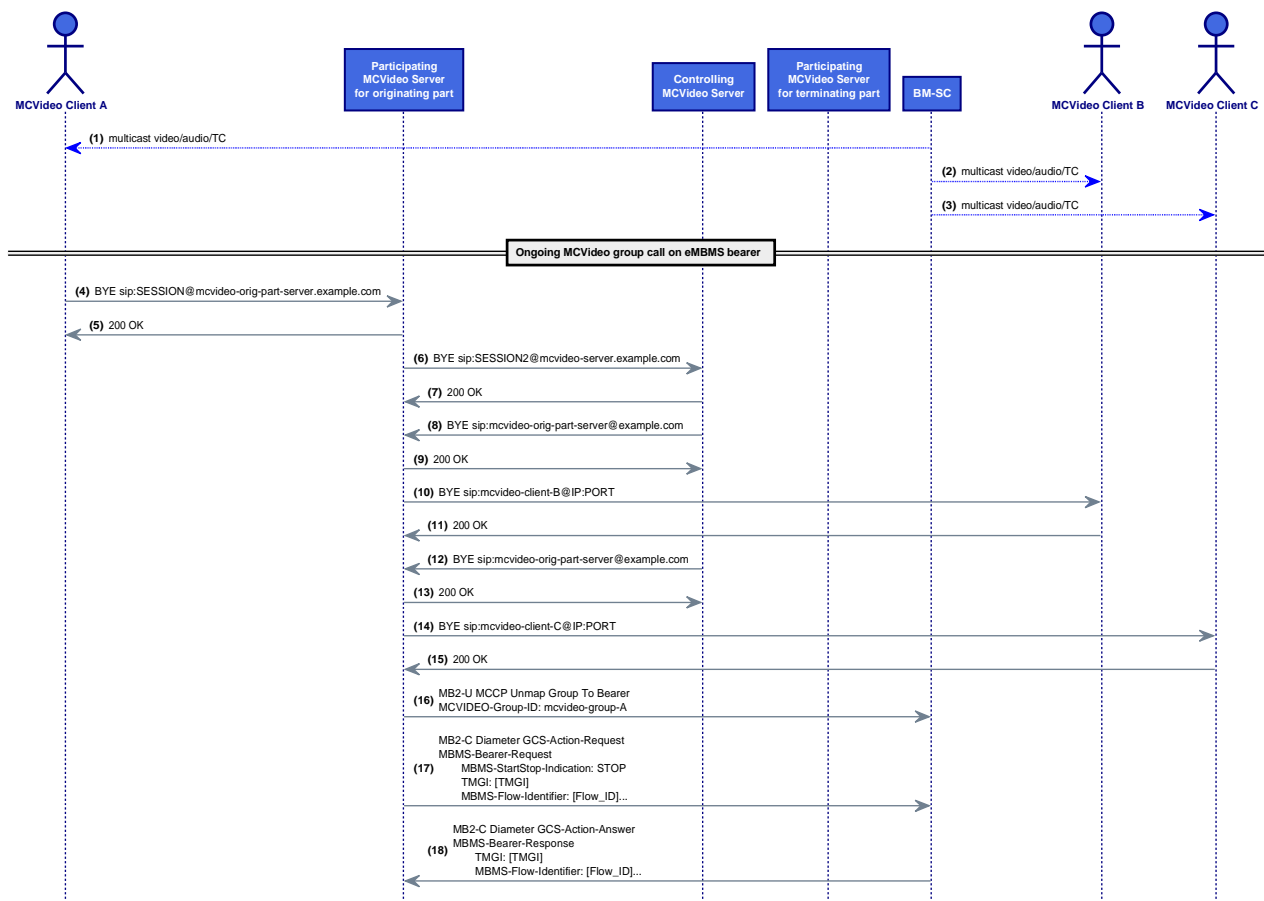
Figure 83i: EMBMS-MCVIDEO/DEACTBEARER/WOTMGIDEA/01 Message Sequence
