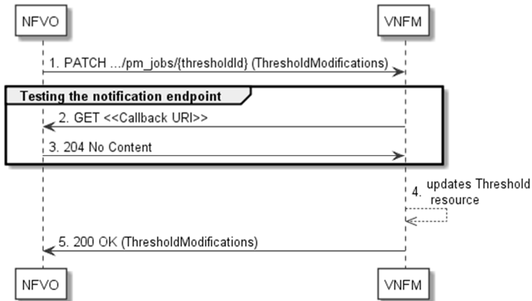
Figure 6.3.5a-1: Flow of threshold callback URI update
