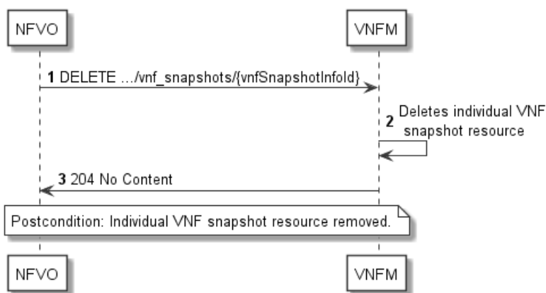
Figure 5.3.18-1: Flow of the deletion of a VNF snapshot resource
